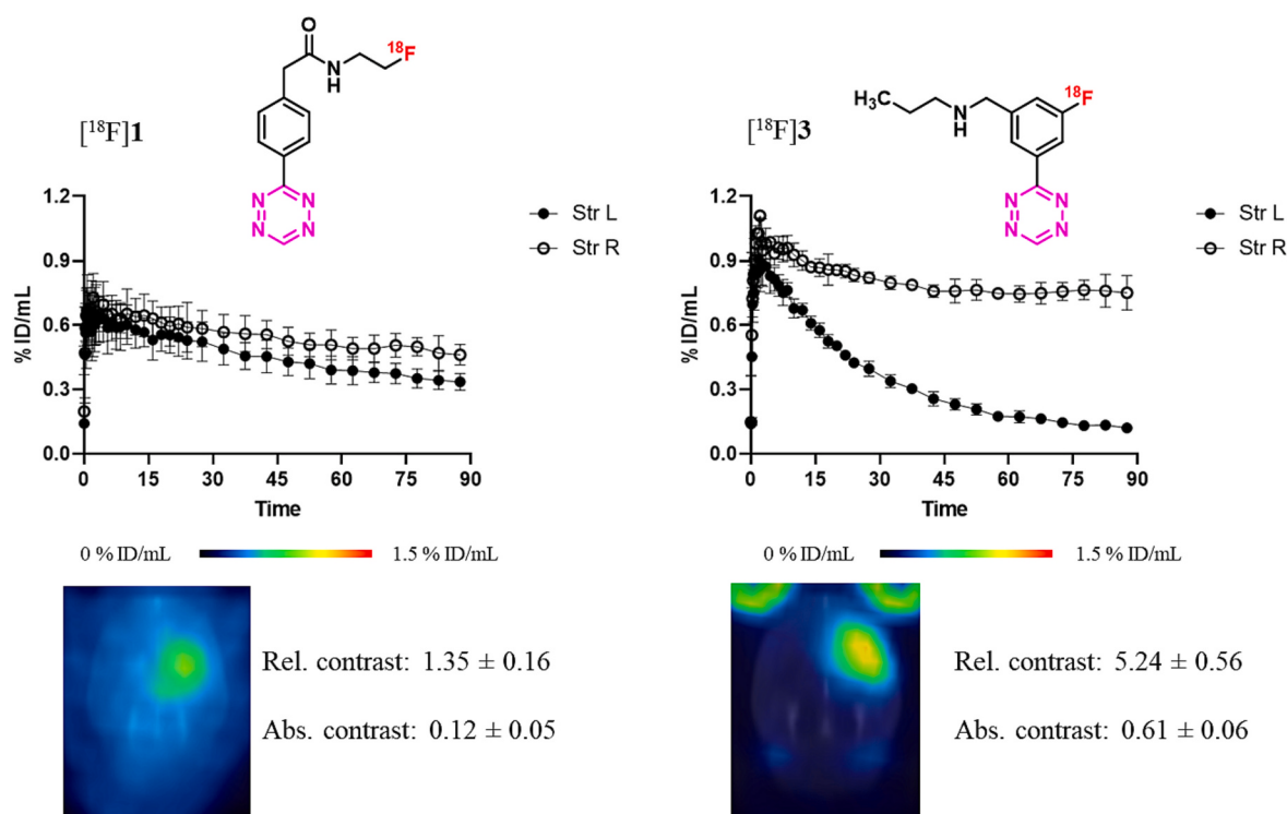
Fig. 4. In vivo click performance of [ 18 F]1 and [ 18 F]3 in the intracerebral TCO-polymer injection model. Upper: Average time-activity curves for left (polymer-free) and right (polymer-injected) striatum (n = 3). Lower: Horizontal sections of summed PET images for 60–90 min post-injection and relative/absolute contrast measurements. The data for compound [ 18 F]3 were previously published data [34].
