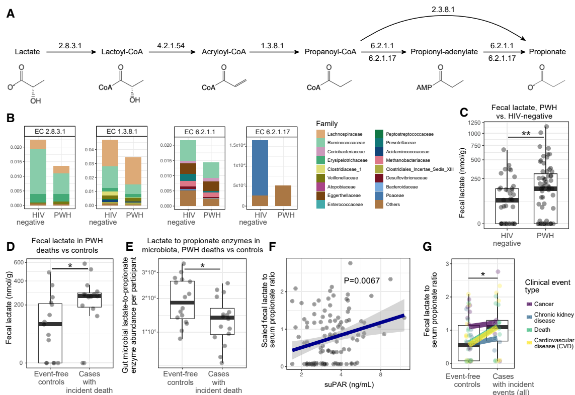
Figure 4. Conversion of fecal lactate to propionate by gut microbes is impaired in PWH and associates with inflammation and future death (A) Lactate-to-propionate conversion pathway (excerpt of KEGG ko00640). EC numbers are shown above transformation lines.
