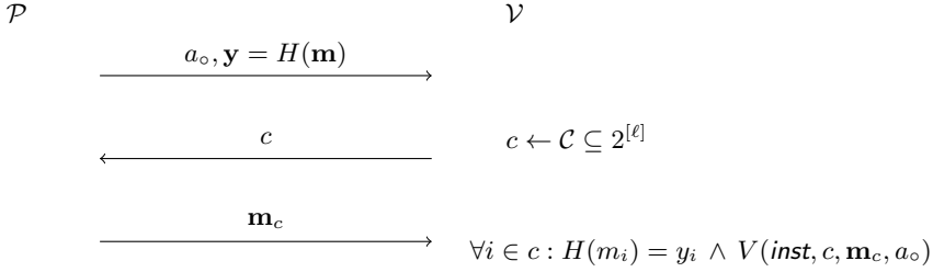
Fig. 2.1. An (ordinary) C&O \Sigma -protocol.
