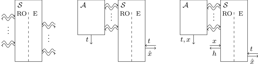
Fig. 4.3. The extractable RO-simulator \mathcal{S} , with its \mathcal{S}.\text{RO} and \mathcal{S}.\text{E} interfaces, distinguished here by queries from the left and right (left), and the games considered in Proposition 4.13 (middle) and 4.14 (right) for \ell = 1 . Waved arrows denote quantum queries, straight arrows denote classical queries.
