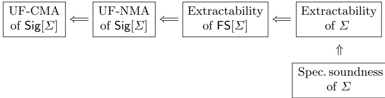
Fig. 4.7. Chain of arguments for proving security of FS signatures.
