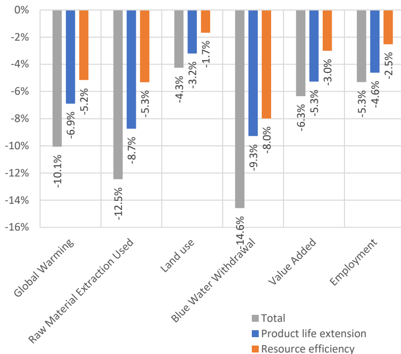
Figure 4: Global potential effects of the CE strategies and their combination
