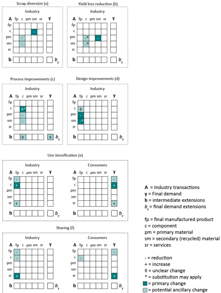
Figure 3: Resource efficiency (RE) modelling blueprints
