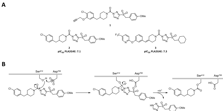
Figure 5.2. Rationale of the design of PLA2G4E probe 1. A) The design of 1 was based on the chemical structure of inhibitors 2 and 3 . pIC_{50} values were determined with gel-based ABPP on PLA2G4E-HEK293T lysate. B) Hypothesized mechanism of PLA2G4E inhibition by 2 . PLA2G4E's nucleophilic residue Ser 412 is activated by Asp 700 and attacks the electrophilic carbonyl of 2 . The triazole moiety leaves, forming a stable adduct of the piperidine moiety on PLA2G4E.
