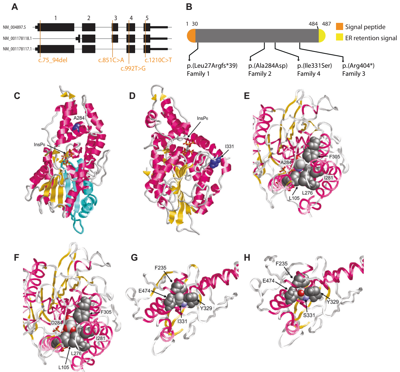
Fig. 2 Molecular modeling. Locations of the variants in MINPP1 gene ( a ) and protein ( b ). Model of the MINPP1 structure ( c–h ) illustrating the effect of truncation and missense variants and the location of the variants on the gene. c Structure of MINPP1 (backbone representation) showing the location of p.A284 (blue) and the bound \text{InsP}_6 substrate (stick representation). Also, the p.Arg404* truncation variant causes the loss of several elements in secondary structure (missing elements are indicated in cyan). d Structure of MINPP1 (backbone representation) showing the location of p.Iso331 (blue) and the bound \text{InsP}_6 substrate (stick representation). e p.Ala284 is buried in the hydrophobic core of MINPP1 . p.Ala284 is colored according to the
