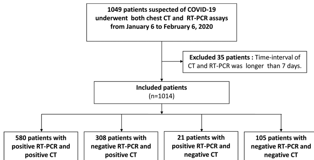
Figure 1: Study flowchart. COVID-19 = coronavirus 2019, RT-PCR = reverse-transcription polymerase chain reaction.
