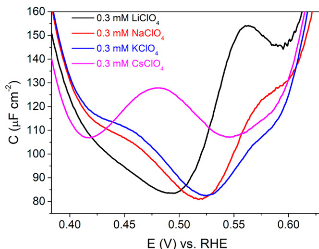
Fig. 5. Comparison between double-layer capacitance curves at pH 4 in 0.1 mM \text{HClO}_4 + 0.3 mM \text{MClO}_4 ( \text{M} = \text{Li}, \text{Na}, \text{K}, and \text{Cs} ).
