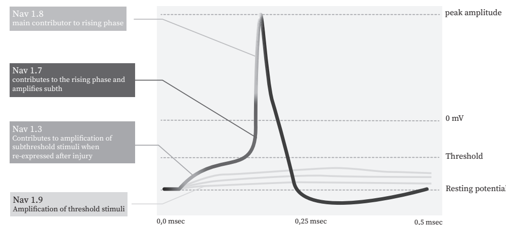
Figure 3 Illustration of unique role of various Nav channels in action potential generation. (Adapted from [40]) (full color version of this illustration on inside of the cover)
