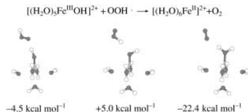
Figure 6. Second step in the hydrogen-abstraction mechanism: a hydrogen is abstracted from the OOH · radical to form the hexaaqua-Fe II complex and O 2 .
