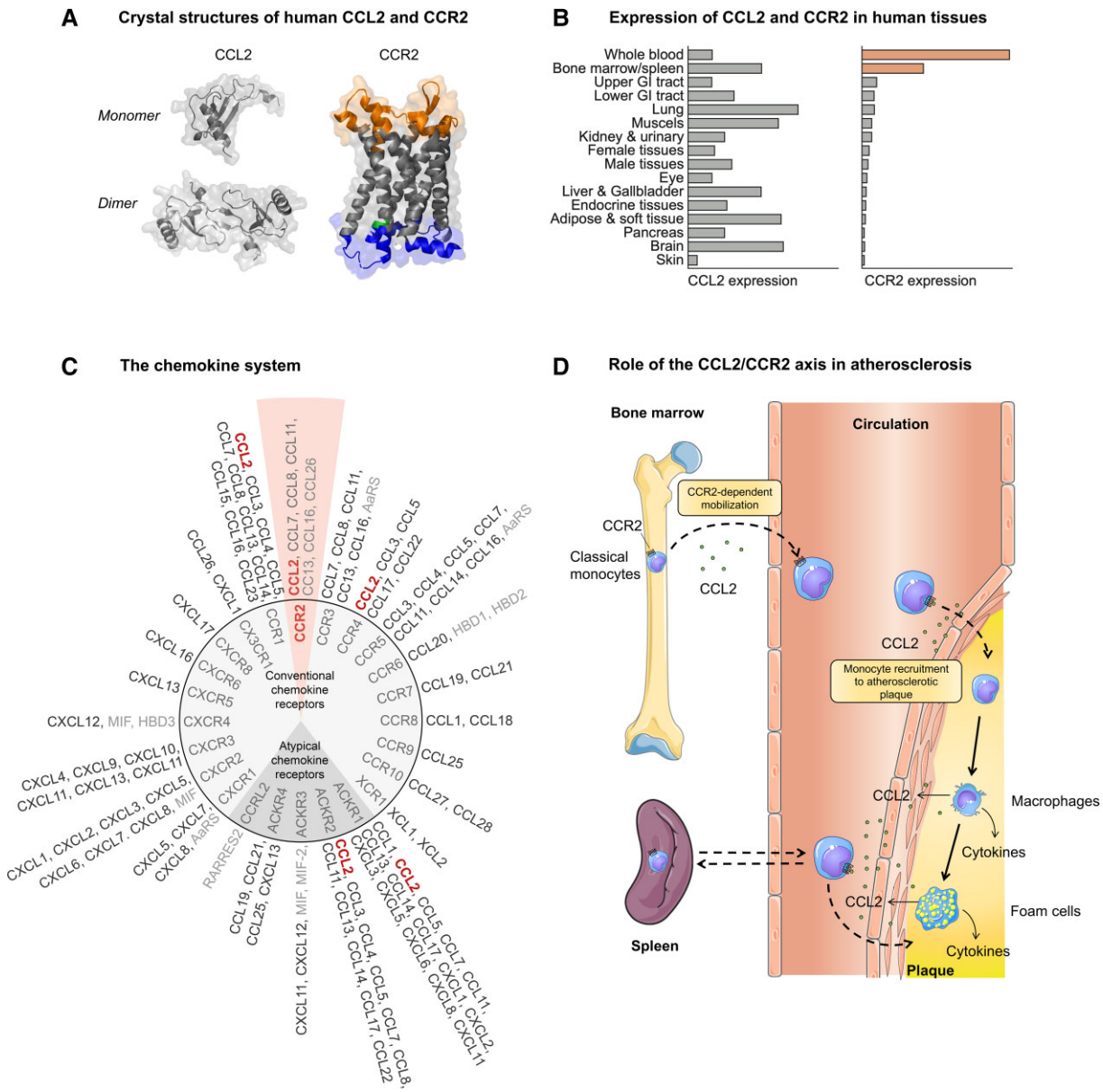
Figure 1 The CCL2–CCR2 axis and its role in atherosclerosis. (A) Shown are the crystal structures of CCL2 and CCR2. CCL2 is depicted both in its monomeric and dimeric forms. The individual structures of CCL2 and CCR2 were created with PyMOL version 2.4.1 and are based on the X-ray structures 1DOK and 5t1a, respectively. 29–32 The intracellular loops of CCR2 are coloured in blue and the G protein activation motif DRY is highlighted in green; extracellular loops are coloured in orange. (B) Expression of CCL2 and CCR2 in human tissues (data extracted from The Human Protein Atlas, https://www.proteinatlas.org ). (C) Network of chemokines and their receptors. Based on differences in their N-terminal cysteine motif, CC-, CXC-, CX 3 C-, and C-type motif chemokines are distinguished, with the CC- and CXC-chemokines representing the predominant classes. 25–28,33–36 With 49 human chemokines interacting with 18 classical chemokine receptors and 5 atypical chemokine receptors, the chemokine system constitutes a large network of ligands and G-protein-coupled receptors. 35–37 Different chemokines can induce distinct responses at the same receptor, while a single chemokine can interact with multiple receptors. This network is further complicated by atypical chemokines (in light grey) such as the human beta-defensins or macrophage migration inhibitory factor, and ligand hetero-oligomerization in an expanded chemokine interactome. 33,38,39 CCL2 and CCR2 are represented in bold red and the CCR2 network with its seven ligands is shadowed in orange. (D) Role of CCL2 and CCR2 in the mobilization of ‘classical’ monocytes from the bone marrow and their recruitment into atherosclerotic lesions.
