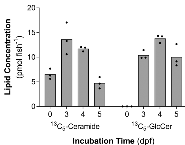
Fig. 4. Incorporation of ^{13}C_5 -sphingosine into the GSL metabolism of zebrafish larvae up to 5 days post-fertilisation. Three samples of five fish each, fed with 20 pmol ^{13}C_5 -sphingosine per fish, were measured.
