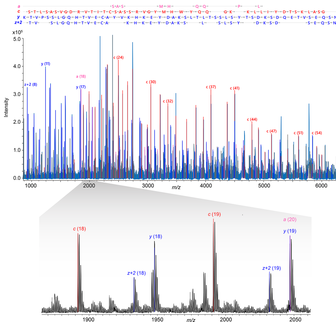
Figure 10. Example of an MD MS mAb analysis: sequencing of the NIST mAb Lc after chromatographic separation with a Bruker rapifleX MALDI-TOF MS based on MALDI-MS/MS. (Top panel) MALDI-MS/MS mass spectrum. Product ion types a , c , y , and z + 2 were assigned. Monoisotopic peak list was obtained by usage of the SNAP algorithm for singly charged ions. (Bottom panel) Expanded view of the full range mass spectrum exhibiting baseline resolution of isotopic distributions. Additional expanded views are in Figure S59.
