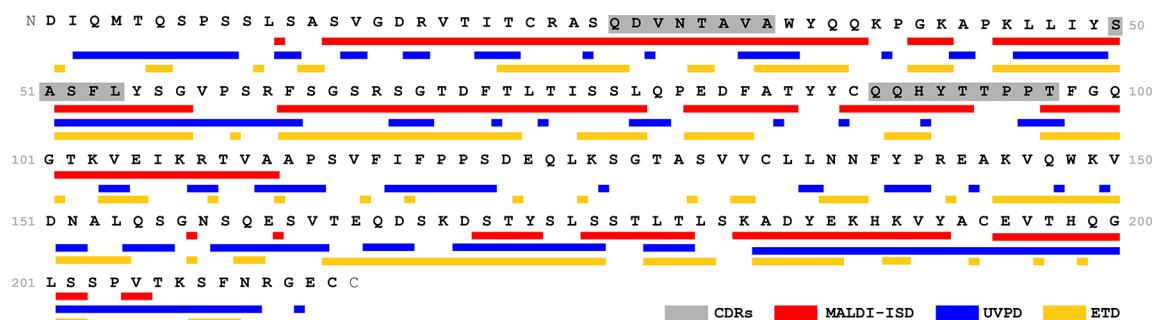
Figure 9. Comparison of sequence coverage (represented by sequence tags) and individual backbone cleavage sites obtained with ESI UVPD, ESI ETD, and MALDI-MS/MS for the Lc of trastuzumab. Included data are from groups 9 (ETD), 14 (UVPD), and 21 (MALDI-MS/MS). See Figures S35, S39, and S41 for more details.
