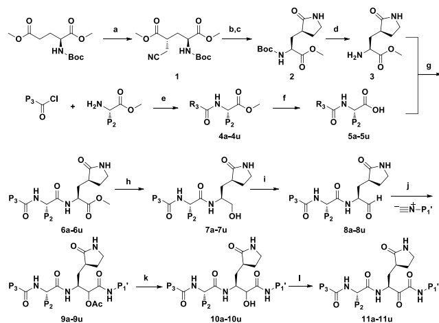
Scheme 1. Synthesis of \alpha -Ketoamides a
