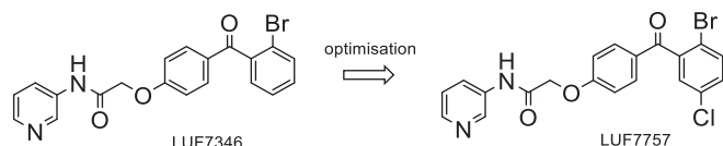
Fig. 1. Optimisation of the substituted benzophenone moiety.
