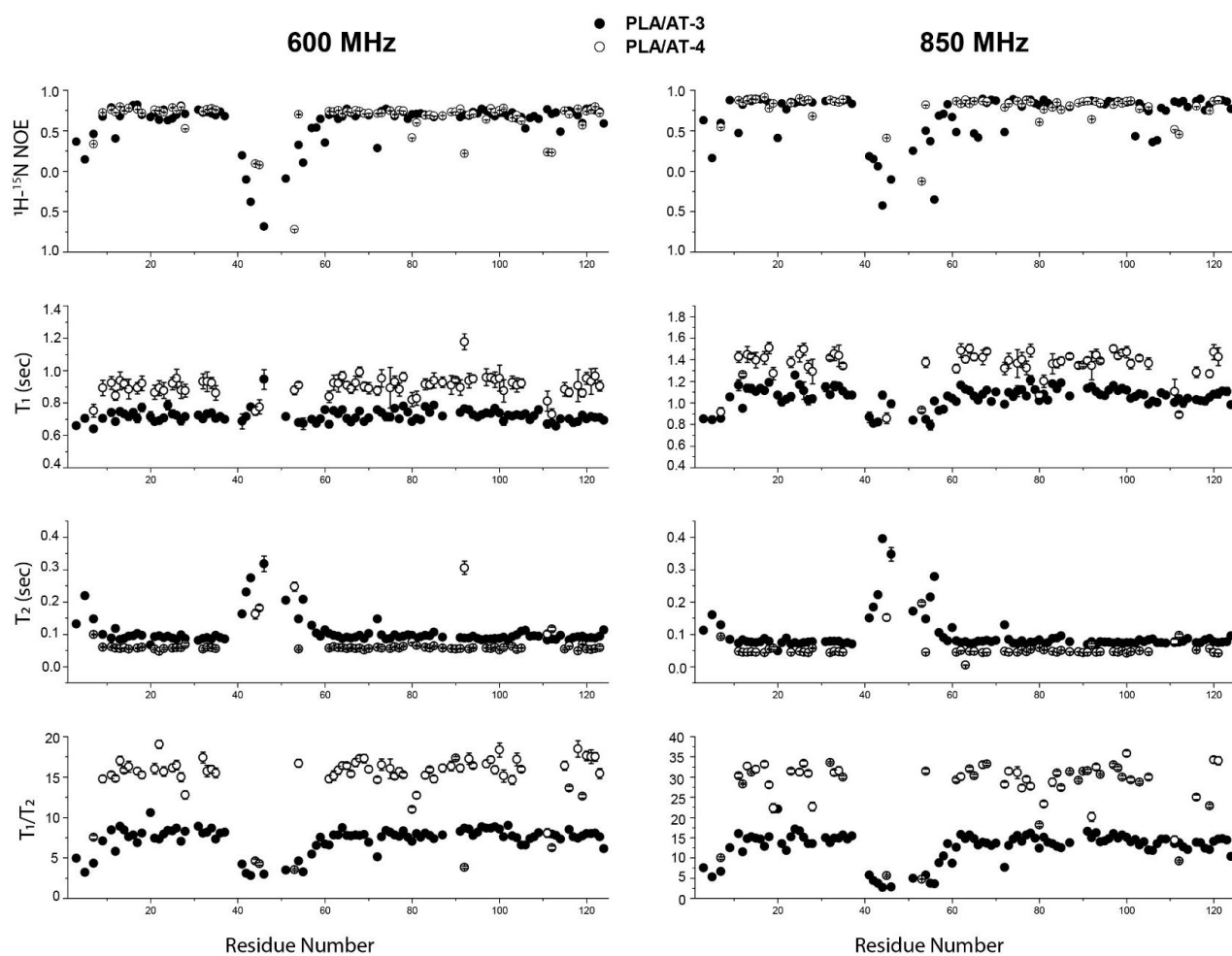
Figure 2.4 Relaxation data for PLAAT3 (solid circles) and PLAAT4 (open circles) at 14 T (600 MHz) and 20 T (850 MHz). The {}^{15}\text{N} -NOE, {}^{15}\text{N} - T_1 , and {}^{15}\text{N} - T_2 as well as T_1/T_2 are plotted against the residue number. Errors were estimated by the Monte Carlo method using 95% confidence level incorporated in Bruker Protein Dynamics software suite.
