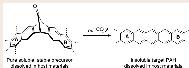
In-situ preparation of a PAH diluted in a solid matrix by photochemical decarbonylation of a precursor.
