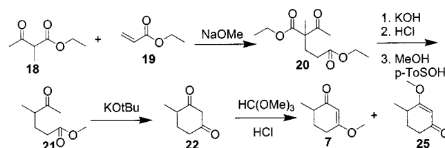
Scheme 4. Synthesis of 4-methyl-1,3-cyclohexanedione
