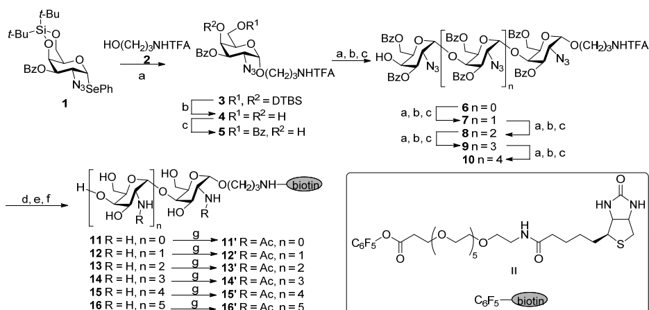
Scheme 1. Chemical synthesis of oligo- \alpha -(1 \rightarrow 4)-galactosamine conjugates. a) 2 , \text{Me}_2\text{S}_2 , \text{MeOTf} , MS 4Å, DCM, for 3 : 81%; 1 , \text{Me}_2\text{S}_2 , \text{MeOTf} , MS 4Å, DCM, for 6 – 10 ; b) 40% aq HF, pyridine; for 4 : 80%; c) \text{BzCl} , pyridine, 0 °C, for 5 : 94%; for 6 : 71%; for 7 : 72%; for 8 : 72%; for 9 : 60%; for 10 : 55%; d) \text{Pd}(\text{OH})_2/\text{C} , \text{Et}_3\text{N} , \text{Boc}_2\text{O} , \text{EtOAc} , atm. \text{H}_2 ; e) 1M \text{NaOMe} , DCM– \text{MeOH} (1:3), then 1 M \text{NaOH} ; f) \text{C}_6\text{F}_5 -biotin, \text{Et}_3\text{N} , DMF, then \text{CF}_3\text{COOH} , for 11 : 71%; for 12 : 62%; for 13 : 53%; for 14 : 48%; for 15 : 72%; for 16 : 53%; g) \text{Ac}_2\text{O} , \text{Et}_3\text{N} , \text{MeOH} , for 11' : 90%; for 12' : 97%; for 13' : 95%; for 14' : 88%; for 15' : 80%; for 16' : 87%.
