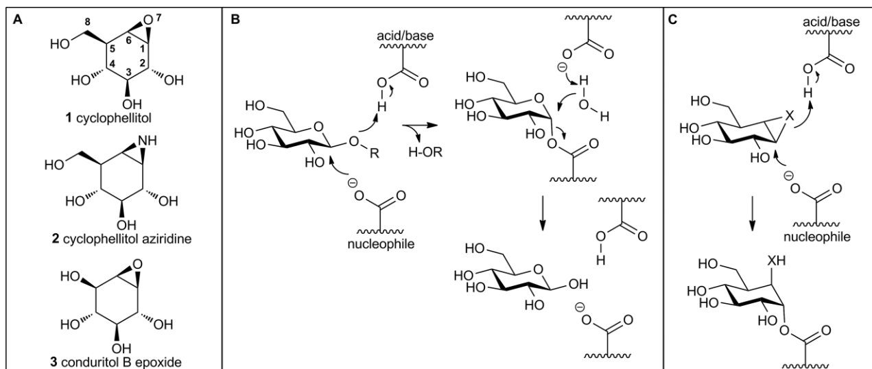
Figure 1. A) Structure of cyclophellitol ( 1 ), cyclophellitol-aziridine ( 2 ) and conduritol B epoxide ( 3 ). B) Mechanism employed by retaining β-glucosidases. C) Mechanism-based, irreversible retaining β-glucosidase inhibition by compounds 1 and 2 (X = O or NH).
