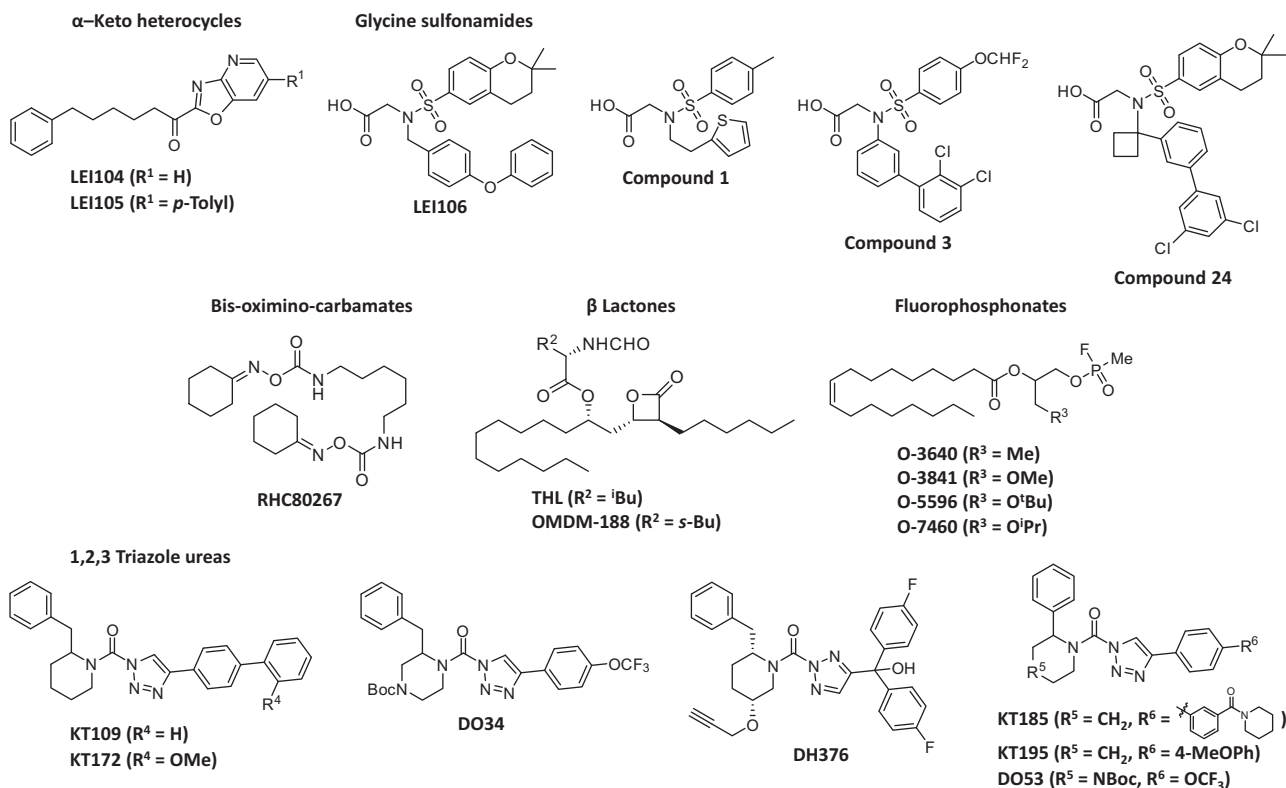
Figure 2. Current DAGL chemotypes and their corresponding inhibitors. 20,28,33,35,41,43,48,55,56,58
