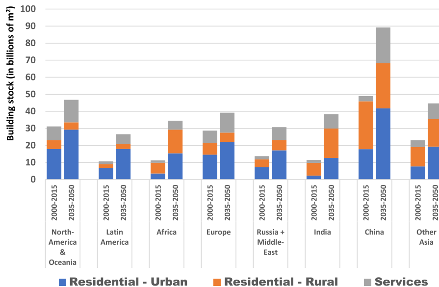
Fig. 2. Regional building stock development for residential & service sector buildings in billion square meters. Bars indicate the average stock in recent history (average of the 2000–2015 period) and by the end of the scenario period (average of the 2035–2050 period). For the per capita floor space demand, see Figure S9 in the SI.
