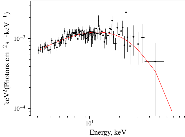
Figure 2. Broadband energy spectrum of the source as observed by NuSTAR in quiescence unfolded with best-fit model and multiplied by energy squared.
