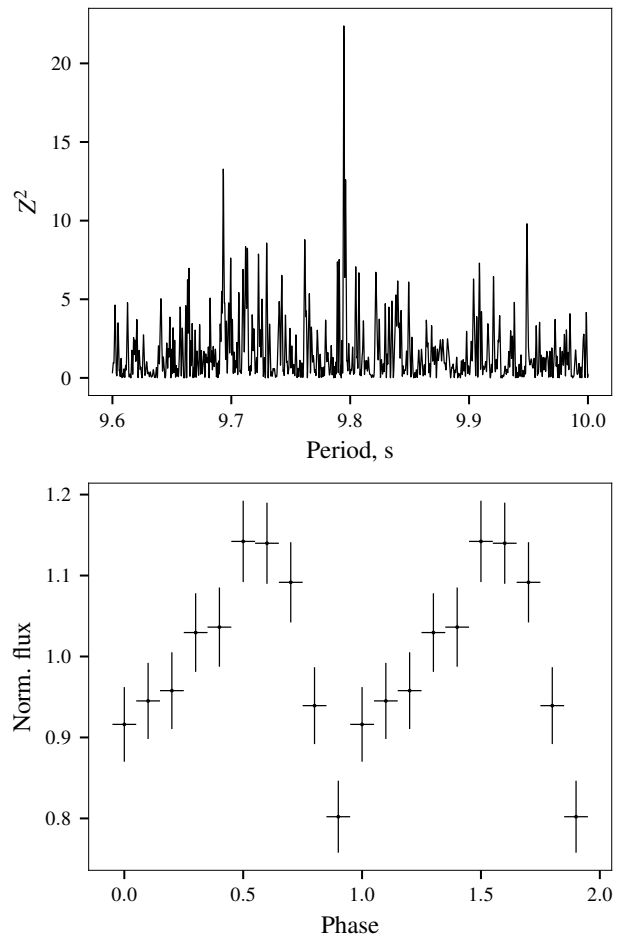
Figure 1. Top: A periodogram for event arrival times for NuSTAR observation 90501310002 (80'' extraction radius, 3-80 keV band). Bottom: Background-subtracted lightcurve for NuSTAR observation 90501310002 in 3-80 keV band folded with best fit period. The pulse profile is plotted two times for clarity.
