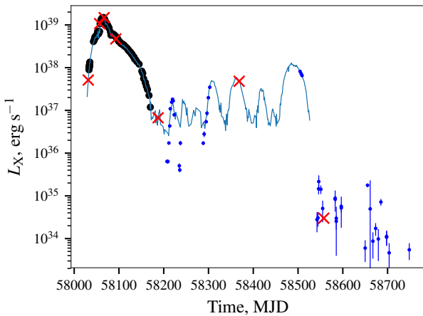
Figure 3. Long-term bolometric lightcurve of Swift J0243.6+6124 as observed by Insight-HXMT (black points), Swift /BAT (blue line), Swift /XRT (blue points), and NuSTAR (red crosses). The dimmest NuSTAR observation marks a hard upper limit on luminosity of “propeller” state, however, accretion likely continues even at lower rates as follows from the observed flux variability revealed by Swift /XRT at later stages.
