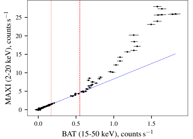
Figure 7. Comparison of count-rates in the soft (2-20 keV) and hard (15-50 keV) energy bands based on daily lightcurves by the Swift /BAT and MAXI missions. At lower fluxes the two bands are well correlated (blue dotted line), however, this is not the case at higher luminosities, where the brightness in the soft band substantially increases. The vertical lines correspond to the transitional luminosities as observed by Insight-HXMT.
