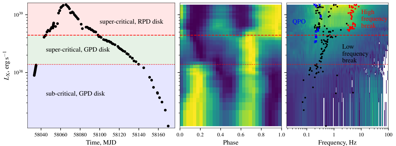
Figure 4. Lightcurve of the source as observed by Insight-HXMT (black points) with color-shading showing the different states of the source. The relevant transition luminosities marked with horizontal lines in all panels. Transition from the sub- to super-critical luminosity is marked by a dramatic change of the pulse profile shape (2nd panel, slices at fixed luminosity are pulse profiles scaled to the same amplitude to emphasize shape evolution). Transition of the accretion disk from GDP to RDP state besides a change in pulse profile shape is also accompanied by a change in power spectrum where amplitude of the aperiodic variability increases in 1-10 Hz frequency range (3rd panel, slices at given luminosity are power spectra multiplied by frequency and scaled as square root to emphasize changes in shape).
