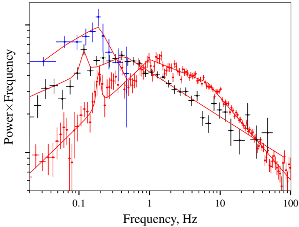
Figure 5. Representative power spectra above (red) and below (black) the transition from GPD to RPD state as observed by Insight-HXMT (arbitrary scaled and multiplied by the frequency to highlight the changes in shape). The low luminosity power spectrum is obtained by combining observations in L_X = 2 - 4 \times 10^{38} \text{ erg s}^{-1} to improve statistics. The second power spectrum is from a single observation slightly above the transition. Estimated white noise and pulsed flux had been subtracted in both cases as described in the text. Note the QPOs feature around 0.1-0.2 Hz. Finally, the power spectrum of the source in quiescence as observed by NuSTAR is also shown (blue points). In the latter case pulsations are not subtracted but do not contribute significantly to the power spectrum.
