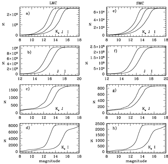
Fig. 4. Cumulative star counts of sources in 0.05 mag bins for the whole catalogue, with detections in three or two bands. From left to right: LMC and SMC. From top to bottom: sources detected in three wave bands, sources detected only in I and J , sources detected only in J and K_s and sources detected only in I and K_s
