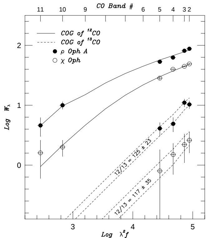
FIG. 5.—Curves of growth for the A – X system of bands in ^{12}\text{CO} (solid lines) and ^{13}\text{CO} (dashed lines) toward \rho Oph A (filled circles) and \chi Oph (open circles). The numbers along the top give v' for the band. The resulting ^{12}\text{CO}/^{13}\text{CO} ratios are also indicated.
