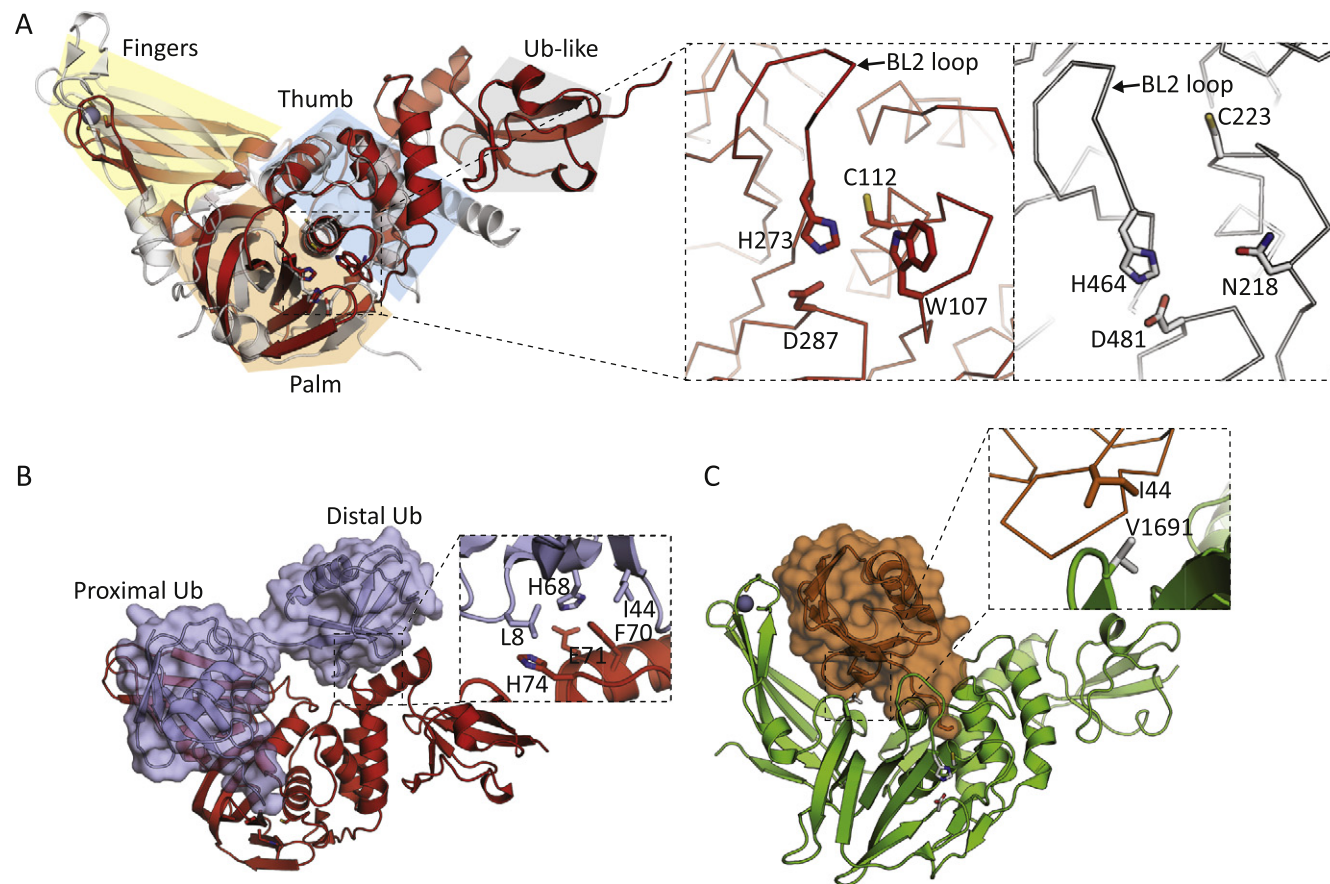
Fig. 5. Crystal structures of zoonotic SARS- and MERS-CoV PL pro domains. (A) Superposition of SARS-CoV PL pro (PDB ID: 2FE8; red) with HAUSP (PDB ID: 1NB8; transparent gray). Thumb, fingers, palm, and UBL domains are indicated with blue, yellow, orange, and gray shading, respectively. Inset is a close-up of the SARS-CoV PL pro (left panel) and HAUSP (right panel) active sites. Backbone atoms are shown as ribbons, and active-site residues are shown as sticks. The BL2 loop is indicated with an arrow. (B) Crystal structure of the SARS-CoV Lys48-linked diUb complex (PDB ID: 5E6J). SARS-CoV PL pro is shown in red, bound to Lys48-linked diUb, shown as a slate cartoon with transparent surface. Inset is a close-up on the hydrophobic interactions occurring between PL pro and the distal domain of Lys48-linked diUb, with relevant residues shown as sticks. (C) Crystal structure of the MERS-CoV PL pro domain in complex with Ub (PDB ID: 4RF0). MERS-CoV PL pro is depicted in green cartoon, and Ub is shown in orange cartoon with transparent surface. Dotted box depicts a close-up of the interaction between MERS-CoV PL pro residue Val1691 and Ub residue Ile44, with residues depicted as sticks.
