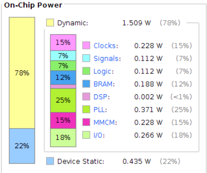
Figure 73: Power consumption of the 4-core MPSoC powering our MPSoC implemented on XKCU3P. Figure generated by Xilinx Vivado 2018.3.
