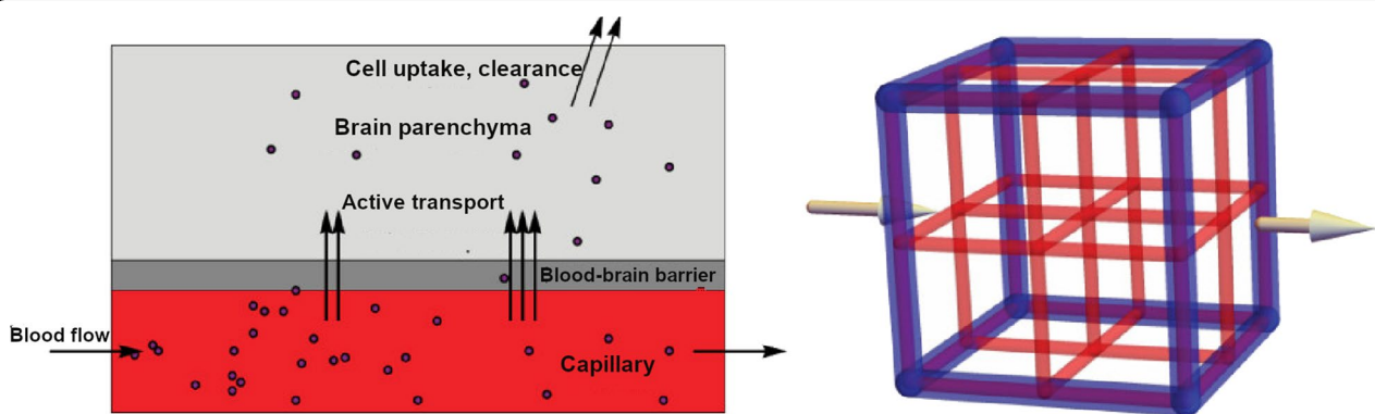
Fig. 10 Model on drug transport within the brain capillaries, active drug transport across the BBB and subsequent metabolism [125]. Spatial differences within the brain are, however, not considered. Left: a simplified model for active drug transport within the capillaries, across the BBB and subsequent metabolism [125]. The black circles represent the drug. Right: a schematic depiction of the lattice refinement process [125]. A cubic lattice (blue) represents a piece of brain tissue with a volume of 1 \text{ cm}^3 . The cubic lattice can be replaced by a network of smaller cubic lattices (red). The larger blue unit and the multiple smaller units fill out the same computational volume. The arrow indicates the direction of the blood flow through the large unit. Both images by [125] are licensed under CC BY 4.0
