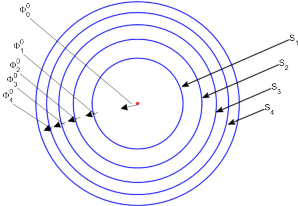
Fig. 9 Circular representation of the Krogh cylinder. A brain capillary (red point in the middle) is surrounded by four layers of brain tissue, represented by subunits S_j (1 \leq j \leq 4) (blue). Here \Phi_0 describes the exchange rate through the BBB and \Phi_j (1 \leq j \leq 4) describes the drug diffusion flux between the brain tissue subunits. Adapted with permission from [111]
