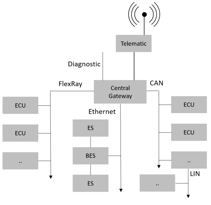
Figure 7.3: A typical schematic in-vehicle network.
