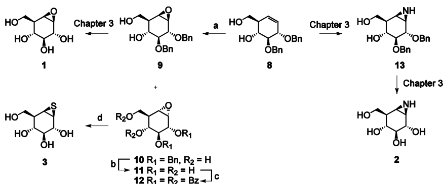
Scheme 1. Synthesis of cyclophellitol 1 , cyclophellitol aziridine 2 and cyclophellitol thiirane 3 .
