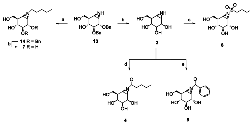
Scheme 2. Synthesis of N -substituted cyclophellitol aziridine 4-7 .
