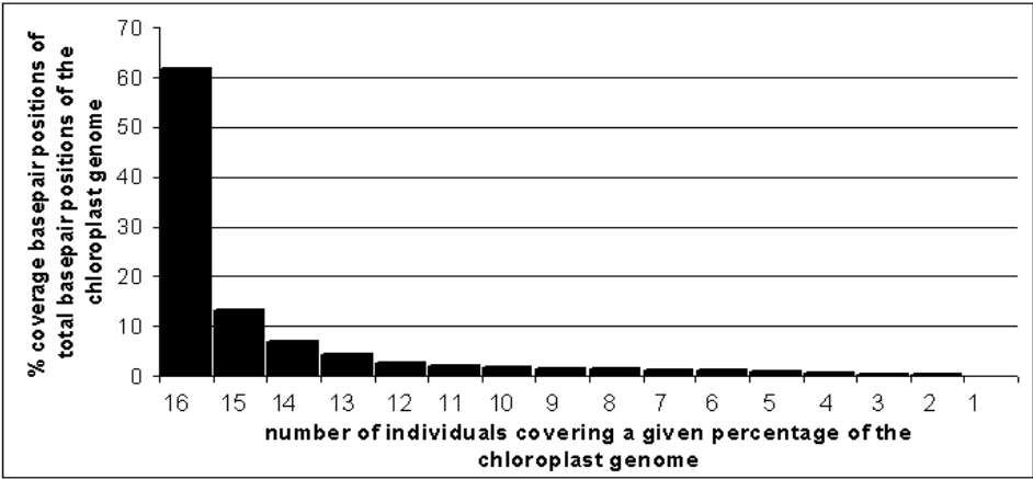
Fig. 3 The column labelled with 1 indicates the number of base pair positions in percentages of total basepair positions that was only covered once in any of these 16 individuals. So, 17 basepairs in the genome were covered by only one individual (less than 0.02 %). To the other extreme the column labelled with 16 indicates the number of base pair positions in percentages of total basepair positions that was covered in all 16 individuals. So, 92804 basepairs were covered by all individuals (more than 60 %).
