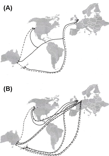
Fig. 1. Different scenarios of the route of introduction from native European Jacobaea vulgaris individuals to invasive regions Australia, New Zealand and North America.
