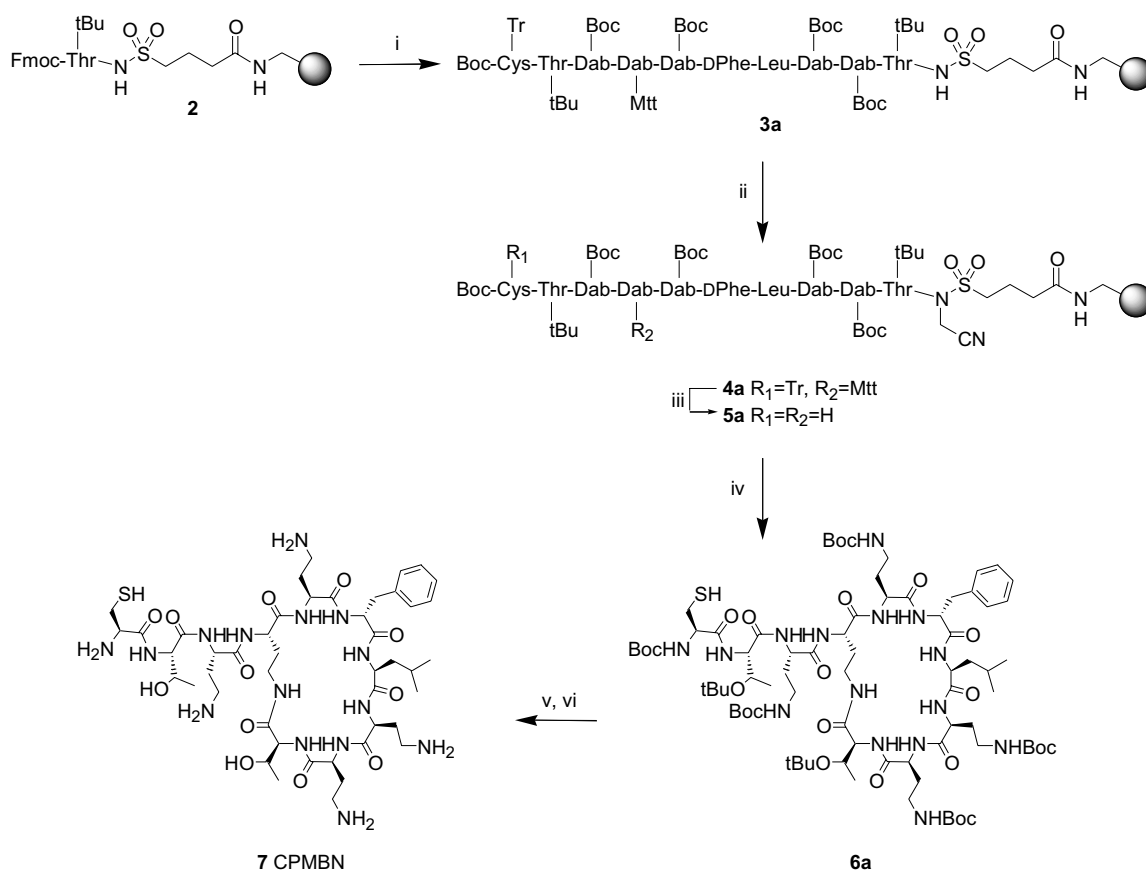
SCHEME 1 | Synthesis of CPMBN. Reagents & conditions: i. Fmoc-based SPPS (see Chapter 2); ii. ICH_2CN , DiPEA, NMP; iii. TFA/TIS/ CH_2Cl_2 5/3/92 (v/v/v); iv. DiPEA, THF; v. TFA/TIS/ H_2O 95/2.5/2.5 (v/v/v); vi. HPLC purification.
