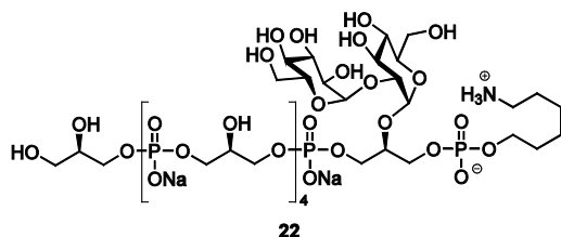
Figure 1. Hexamer 22.
