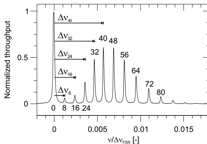
Figure 5.4: Spectral detail of the fundamental mode and the nearest clump of peaks. The almost 8-fold degeneracy makes the difference in mode number between two subsequent modes equal to 8. \Delta\nu_m is the distance between the fundamental mode m = 0 and mode m .
