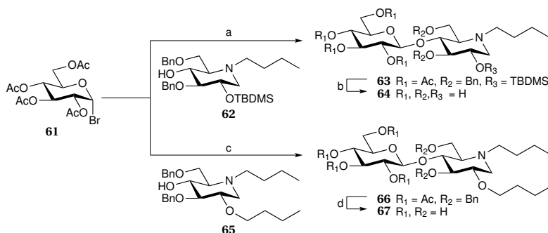
Scheme 1.4: Synthesis of \beta -glucocerebrosidase inhibitors. 58
