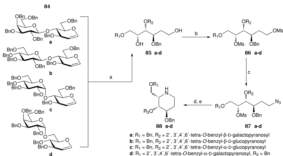
Scheme 1.8: Synthesis of glycosylated imonosugars via D-lactal ( 84a ), D-cellobial ( 84b ), D-maltal ( 84c ) and D-melibial ( 84d ). 63
