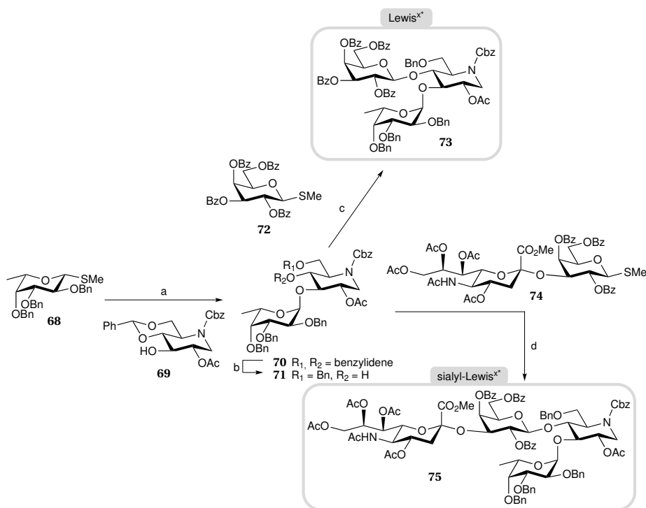
Scheme 1.5: Synthesis of Lewis x 73 and sialyl-Lewis x 75 . 59
