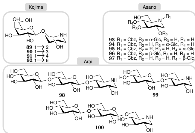
Figure 1.4: Structures of glycosylated iminosugars described in section 1.2.2.
