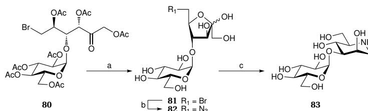
Scheme 1.7: Synthesis of glucosidase inhibitor 83 . 61,62
