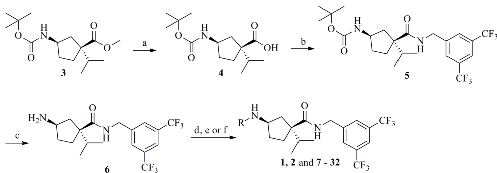
Scheme 1. Synthesis of CCR2 antagonists. Reagents and conditions: (a) 4 M LiOH aqueous, MeOH, reflux, 4 h, 91%; (b) 3,5-bis(trifluoromethyl)benzylamine, PyBroP, N , N -diisopropylethylamine (DiPEA), N , N -dimethylaminopyridine (DMAP), DCM, room temperature, 24 h, 83%; (c) TFA, DCM, room temperature, 1 h, 85%; (d) corresponding ketone, (AcO) 3 BHNa, AcOH, DCE, room temperature, 18 h, 21–86% (compounds 1 , 2 , and 11 , 12 ); (e) corresponding alkylating agent, DiPEA, CH 3 CN, 60 °C, 2 h, 14–54% (compounds 7–9 ); (f) for array synthesis, corresponding ketone, 5-ethyl-2-methylpyridine borane (PEMB), AcOH, N -methylpyrrolidone (NMP), 65 °C, 24 h (compounds 10 and 13–32 ).
