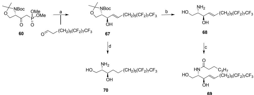
Scheme 1.16 Synthesis of fluorine-containing sphingolipids.
