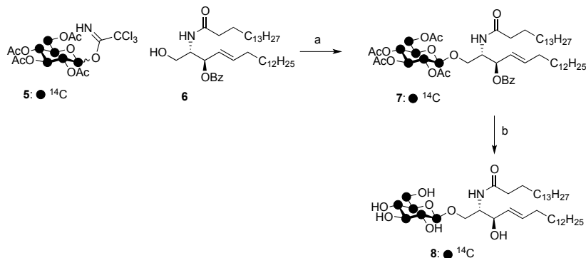
Scheme 1.2 Synthesis of 14 C-glucosylceramide.
