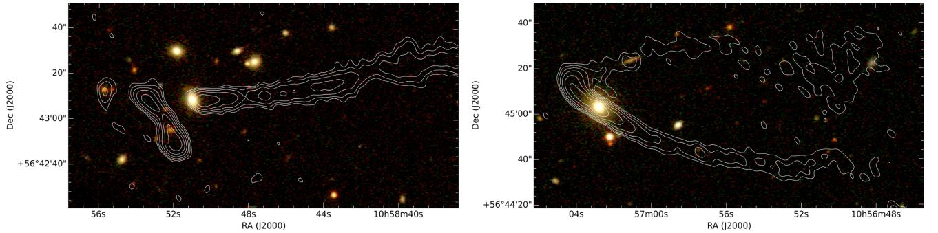
Figure 4. SDDS g, r, i optical images overlaid with GMRT contours at 610 MHz. The levels are [3, 6, 12, 24, 48, 96] \times \sigma where \sigma = 20 \mu\text{Jy beam}^{-1} . Left: the optical source associated with the HT GRG is the elliptical galaxy SDSS J105851.01+564308.5 at a redshift of z \approx 0.139 , within Abell 1132. The double source to the east of the HT is likely associated with the background galaxy SDSS J105852.18+564255.3 at a redshift of z \approx 0.496 . Right: the optical source associated with the WAT is the elliptical galaxy SDSS J105702.79+564503.1 at a redshift of z \approx 0.136 , within Abell 1132.
