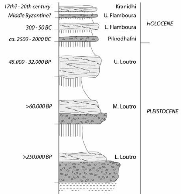
Fig. 6.23 Quaternary alluvial sequence from southern Argolid (Peloponnese). Cobbles with a chaotic structure indicate debris flows, whilst stratified gravels are streamflood deposits; blank zones are overbank loams and vertical lines denote soil profiles. Although the dates give only approximate ages, they do highlight an apparent discontinuity in alluviation events. Modified after van Andel et al. 1986: fig. 4
