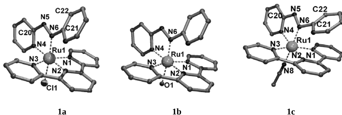
Fig.2.2. PLATON projections of the cations [\text{Ru}^{\text{II}}(\text{apy})(\text{tpy})\text{L}]^{n+} ( \text{L} = \text{Cl}^- , \text{H}_2\text{O} , \text{CH}_3\text{CN} ) ( 1a-c ), with numbering of major atoms. Hydrogen atoms and counter ions have been omitted for clarity.
