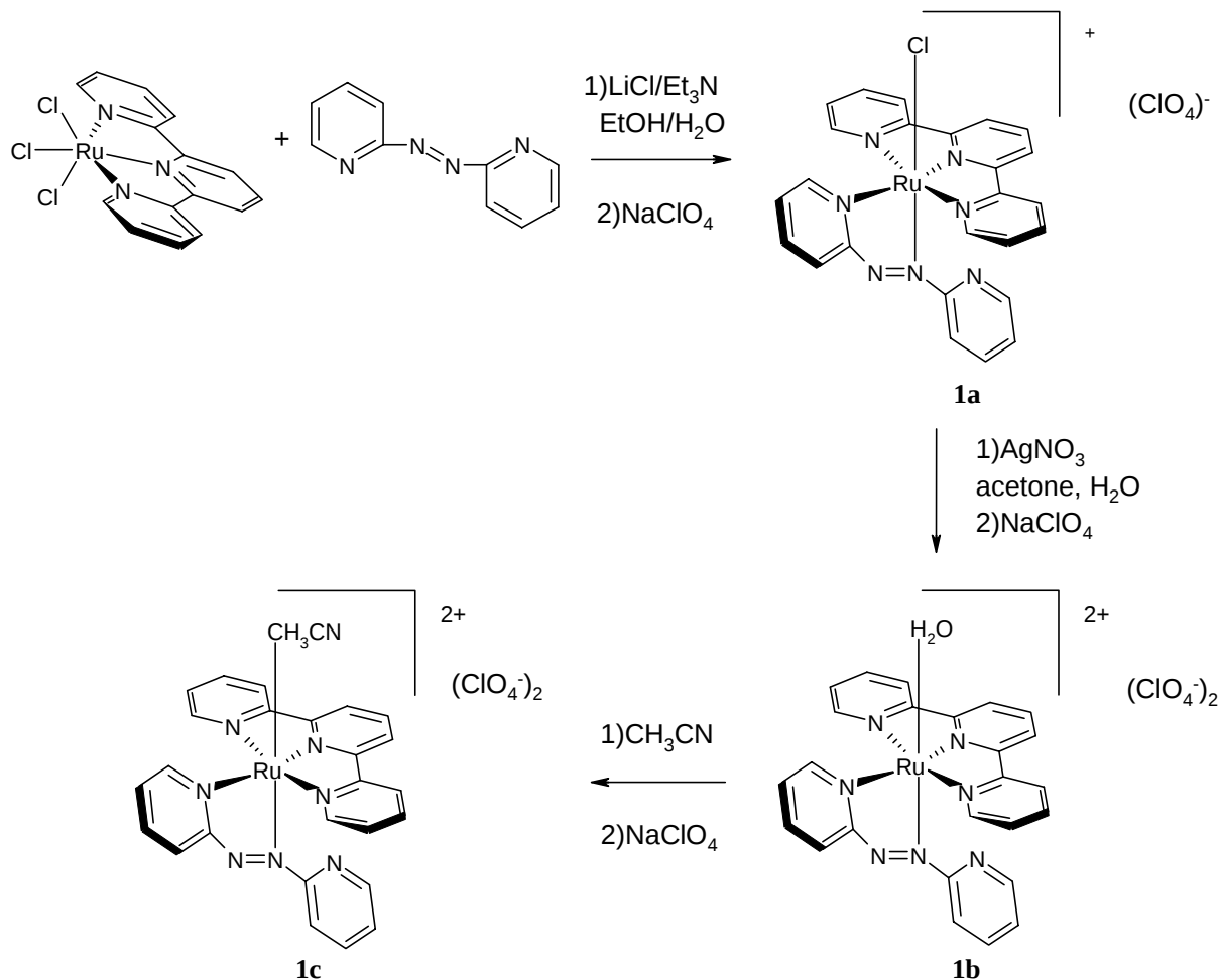
Fig.2.1. Scheme of the synthesis of the [\text{Ru}(\text{apy})(\text{tpy})\text{L}](\text{ClO}_4)_{(2-n)} compounds.
