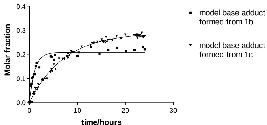
Fig.3.4. Formation of the model base adduct from two ruthenium complexes ( 1b and 1c ).
