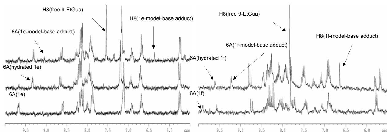
Fig.4.3. ^1\text{H} NMR studies of the reactions 1e + 9-EtGua (left) and 1f + 9-EtGua in \text{D}_2\text{O} (right). The spectra on the left show the complex 1e in \text{D}_2\text{O} at time = 0 (below), the complex 1e in \text{D}_2\text{O} at time = 24 h (centre) and the mixture 1e + 9-EtGua at time = 24 h (above). The spectra on the right show the mixture 1f + 9-EtGua at time = 30 min (below) and at time = 24 h (above). The peaks assigned to the proton 6A in each complex are labeled, as well as the peaks assigned to the proton H8 of 9-EtGua, both in the free ligand and in the Ru-model base adduct.
