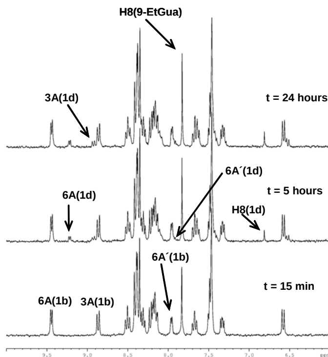
Fig.3.2. ^1\text{H} NMR study over 24 h of the reaction between the ruthenium polypyridyl complex [\text{Ru}(\text{apy})(\text{tpy})(\text{H}_2\text{O})]^{2+} ( 1b ) and the DNA model base 9-ethylguanine in \text{D}_2\text{O} at a 1:2 ratio. Some selected peaks have been labeled with their assignments.
