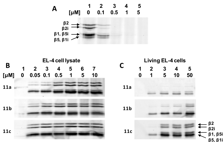
Figure 2. Competition study azidomycin and labeling profile of 11a-c .
