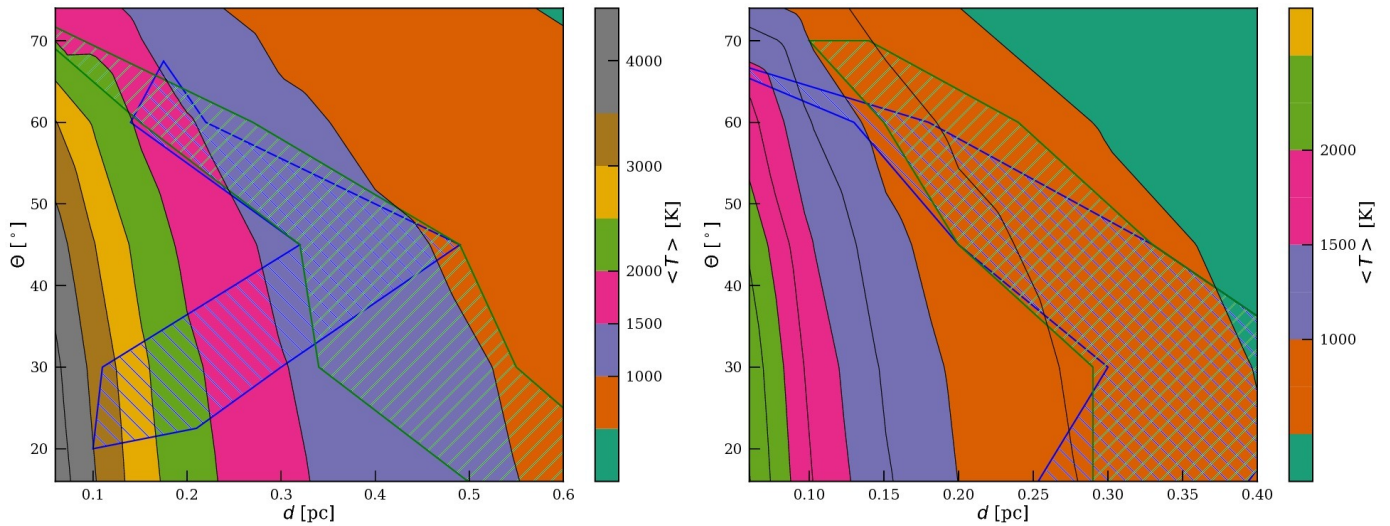
Fig. 14. Peak mean temperature of the disk (contours) due to the supernova radiation as a function of the distance to a supernova ( d in parsec) and the impact angle ( \Theta in degrees, measured from the disk’s angular-momentum axis). The adopted type IIp supernovae, SN11aof (left) has a peak luminosity of 1.1 \times 10^{43} erg/s and SN10a (right) has a peak luminosity of 2.3 \times 10^{42} erg/s. The two shaded regions indicate the range in distance for which the Sun’s obliquity is consistent with the currently observed value of 5^\circ.6 \pm 1^\circ.2 (blue with “/” hashes), and for which the disk is truncated to 42–55 au (green with hashes). This area is indicated in Fig. 12 with a blue polygon. The most promising part of parameter space is where the two hashed areas overlap because for there both criteria are met.
