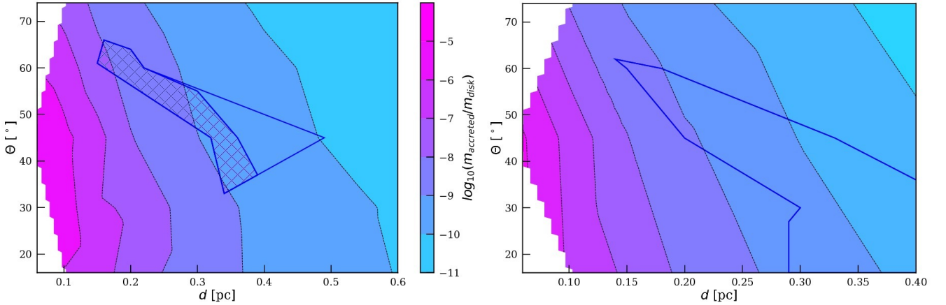
Fig. 12. Disk enrichment mass-fraction as function of the distance to the supernova and its angle with respect to the proto-planetary disk's rotation axis for SN 11aof (left) and SN 10a (right). The colored contours give the amount of accreted mass from the supernova remnant as fraction of the mass of the surviving disk (scale to the right). The enclosed and shaded regions are as in Fig. 11. The small top-left area of the hashed region which overlaps with an enrichment of at least m_{\text{shell}}/M_{\text{disk}} \gtrsim 10^{-3} satisfies all the criteria of the model. The absence of a hashed region in the left panel indicates that there is no consistent solution across all requirements in our simulations for SN 10a.
