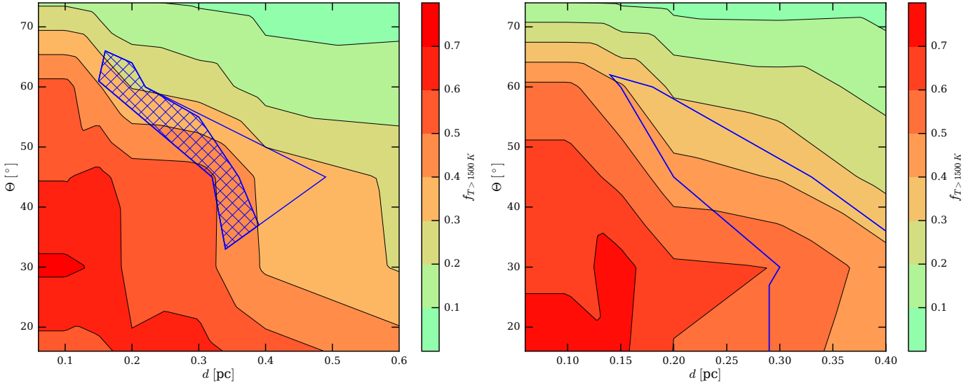
Fig. 11. Fraction of the surviving disk that is heated to a temperature \gtrsim 1500 K by the supernova blast wave (scale to the right) for SN 11aof (left) and SN 10a (right). The enclosed area indicates the initial parameter space for which the observed obliquity and the disk size are satisfactory reproduced by the simulations (see Fig. 7). The hashed subset of this area indicates for which parameters the disk is also heated to a temperature \gtrsim 1500 K by the supernova radiation. The non-hashed area to the lower right indicates for which parameters the disk is sufficiently truncated and tilted by the blast wave but the supernova flash-induced temperature is insufficient to melt corundum.
