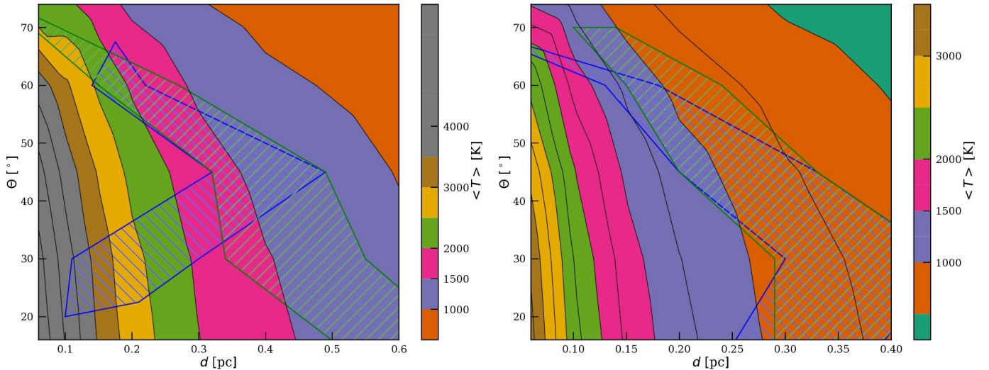
Fig. 7. Peak mean temperature of the disk (contours) due to the supernova radiation as a function of the distance to a supernova ( d in parsec) and the impact angle ( \Theta in degrees, measured from the disk’s angular-momentum axis). The adopted type IIp supernovae, SN11aof (left) has a peak luminosity of 1.1 \times 10^{43} erg/s and SN10a (right) has a peak luminosity of 2.3 \times 10^{42} erg/s. Evaporation of the bulk of the solids in the proto-planetary disk is achieved when the irradiation heats it to a mean temperature of \gtrsim 1500 K. The two shaded regions indicate the range in distance for which the Sun’s obliquity is consistent with the currently observed value of 5^\circ.6 \pm 1^\circ.2 (blue with “\” hashes), and for which the disk is truncated to 42–55 au (green with “/” hashes). This area is indicated in Fig. 11 and Fig. 12 with a blue polygon. The most promising part of parameter space is where the two hashed areas overlap because for there both criteria are met.
