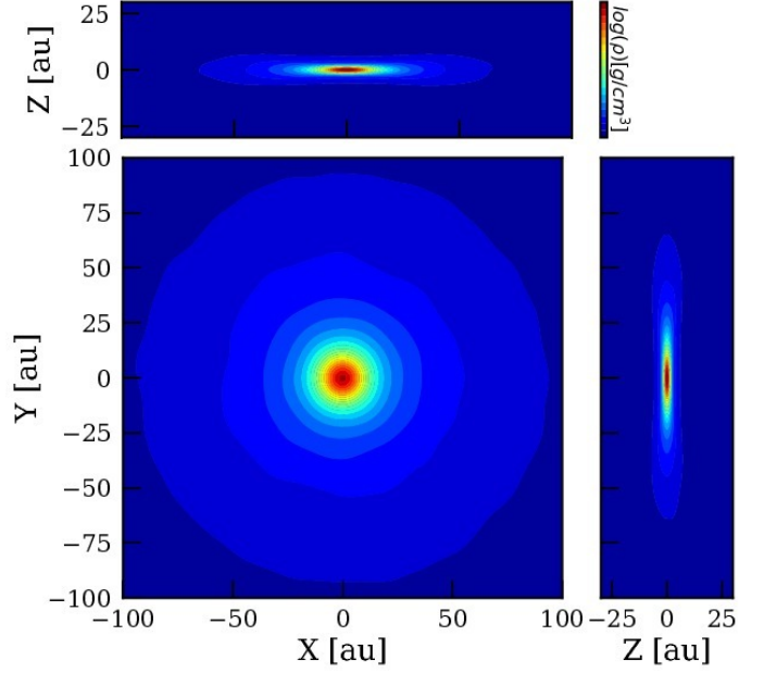
Fig. 2. Mid-plane density distribution of the protoplanetary disk with a top view in the middle and side views to the right and top. The density is color coded, the coding scheme is presented to the top right of the figure. The density extremal range from 10^{-12.9} g/cm 3 to 10^{-9.97} g/cm 3 .
