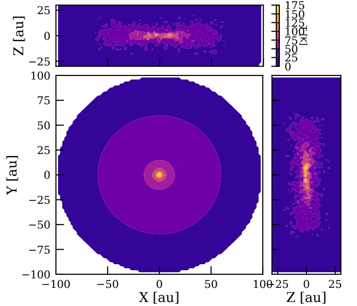
Fig. 3. Top view of the protoplanetary disk from three sides, the top view ( x - y ) image in the middle and two side aspects to the right and top. The colors represent temperature, and the coding is represented by the bar to the top right.
