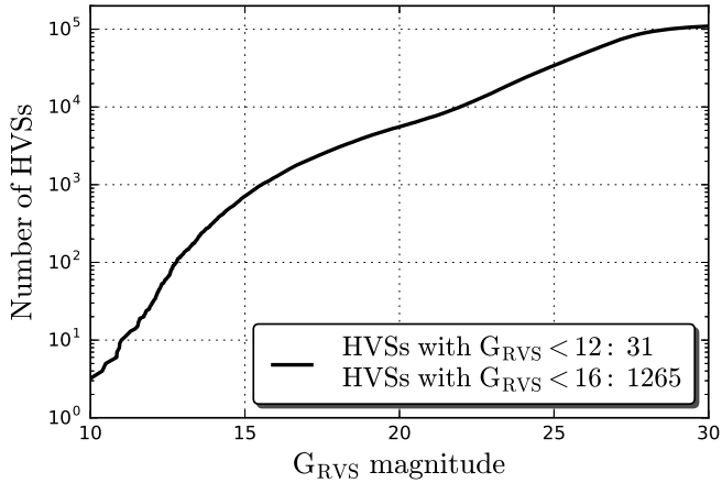
Figure 15. MBHB catalogue: cumulative distribution of HVs magnitudes in the Gaia G_{\text{RVS}} passband.
