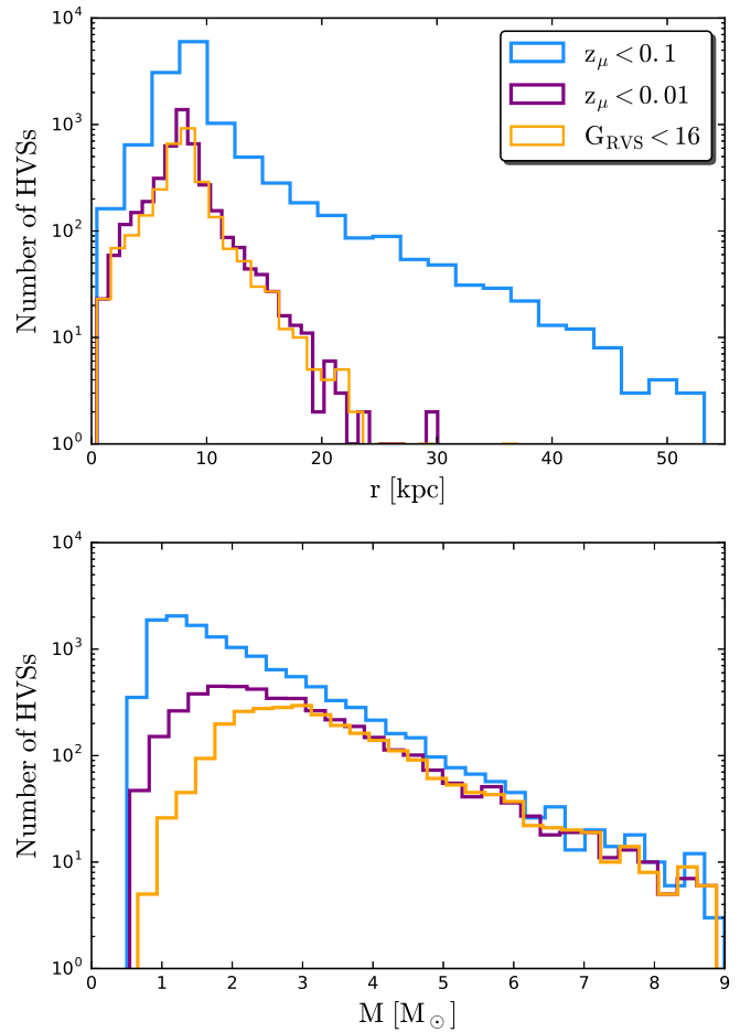
Figure 10. HILLS catalogue: heliocentric distance (top) and mass (bottom) distribution of the HVSs with a relative error on total proper motion below 10% (blue), 1% (purple), and with a radial velocity measurement by Gaia (yellow).
