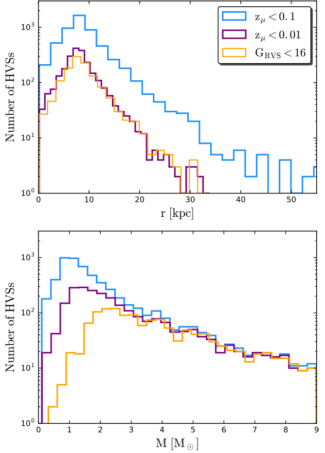
Figure 16. MBHB catalogue: heliocentric distance (top) and mass (bottom) distribution of the HVs with a relative error on total proper motion below 10% (blue), 1% (purple), and with a radial velocity measurement by Gaia (yellow).
