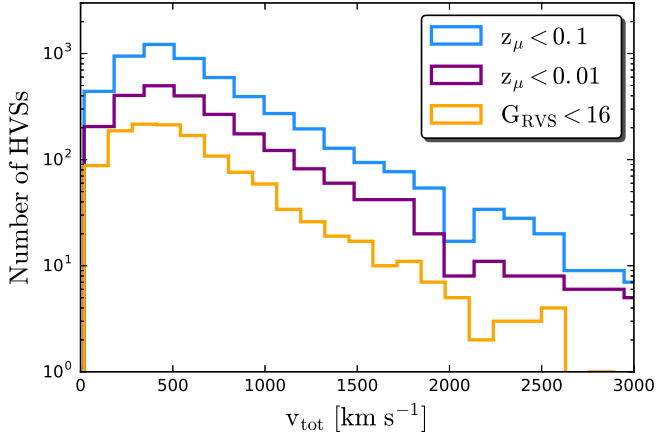
Figure 14. MBHB catalogue: total velocity (in the Galactocentric rest frame) of HVs.
