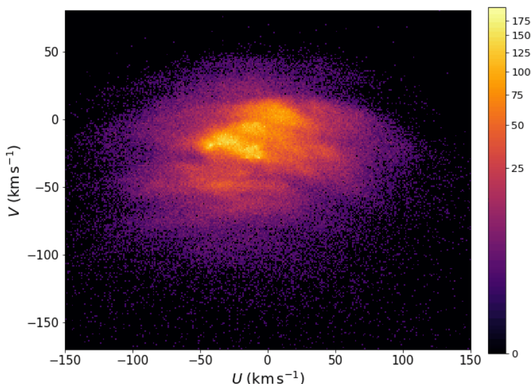
Fig. 22. Velocity plane of the stars in the solar neighbourhood. We show a 2D histogram of the velocity with a bin of 1 \text{ km s}^{-1} , thus, the colour scale indicates the number of stars per (\text{km s}^{-1})^2 .
