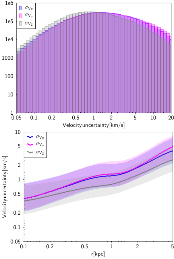
Fig. 4. Top: Histogram of velocity uncertainties in the Galactic cylindrical reference system ( V_R , V_\phi , V_z ) for the main sample. Bottom: Median uncertainties in velocity as a function of the heliocentric distance for the main sample. The 25% and 75% quartiles are shown as colour-shaded areas.
