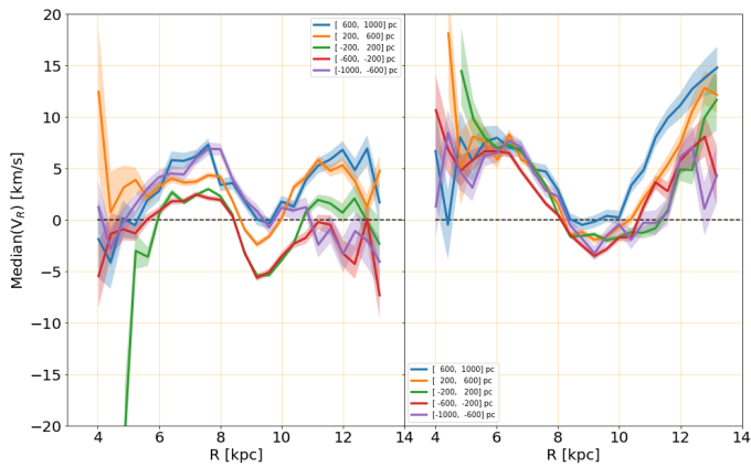
Fig. 12. Median radial velocities, \tilde{V}_R , of the giant sample as a function of Galactic radius for two azimuth slices: [-30, 0] degrees (left), and [0, +30] deg (right). The curves correspond to different Z layers, defined in the legend. The shaded areas represent the \pm 1 - \sigma uncertainties on the median radial velocities.
