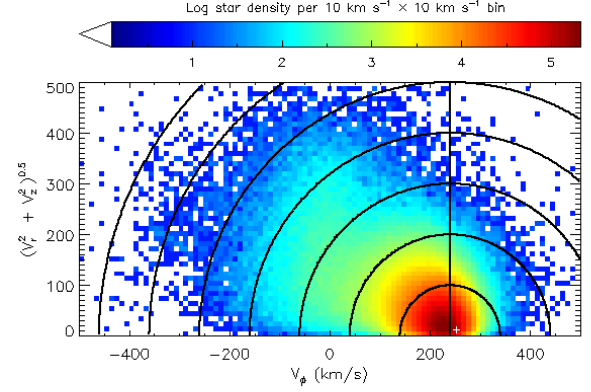
Fig. 5. Toomre diagram of the main sample. The vertical line crosses the LSR at (V_R, V_\phi, V_z) = (0, 240, 0) \text{ km s}^{-1} . The white dot is the peculiar velocity of the Sun: (V_R, V_\phi, V_z) = (11.10, 252.24, 7.25) \text{ km s}^{-1} . The concentric circles show the total peculiar velocity, centred on the LSR. The traditional use of the Toomre diagram to classify stars into stellar populations is complicated by the great range of the Galactic radius of the sample (Fig. 3) and the possibility that both the mean V_\phi of the thin disc and the V_\phi lag between the thin and thick disc may vary with Galactic radius. Nevertheless, it shows that the sample is dominated by the thin disc. In the solar neighbourhood, the thin disc has an azimuthal velocity close to the LSR, and the thick disc lags behind by a few tens of \text{km s}^{-1} .
