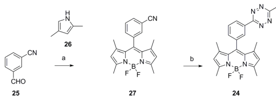
Scheme 4. Synthesis of BODIPY-tetrazine. Reagents and conditions: (a) i . TFA (catalytic), DCM; ii . DDQ; iii . DIPEA, \text{BF}_3 \cdot \text{OEt}_2 ; 42%; (b) i . \text{Zn}(\text{OTf})_2 , \text{CH}_3\text{CN} , \text{NH}_2\text{NH}_2 , 60 °C; ii . \text{NaNO}_2 ; 0.3%.
