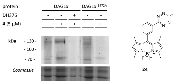
Figure 4. In situ two-step labeling of DAGLα overexpressed in U2OS cells with probe 4 and BODIPY-tetrazine 24 (10 μM).
