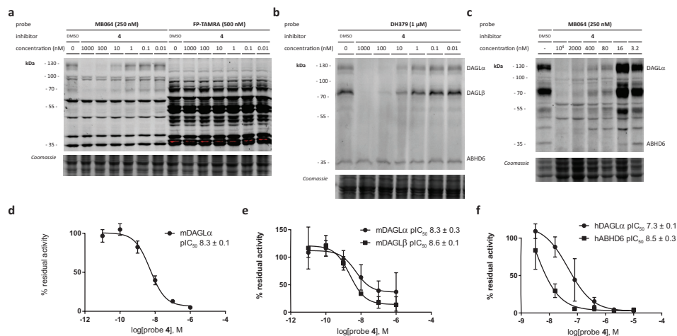
Figure 3. Activity-based protein profiling of probe 4 in mouse brain membrane proteome against (a) MB064 and FP-TAMRA and (b) DH379. (c) In situ treatment of U2OS cells transfected with DAGLα. (d) Quantification of residual DAGLα activity as measured with MB064 in mouse brain. (e) Quantification of residual DAGLα and DAGLβ activity as measured with DH379 in mouse brain. (f) Quantification of residual DAGLα and ABHD6 activity as measured with MB064 in U2OS-DAGLα cells.
