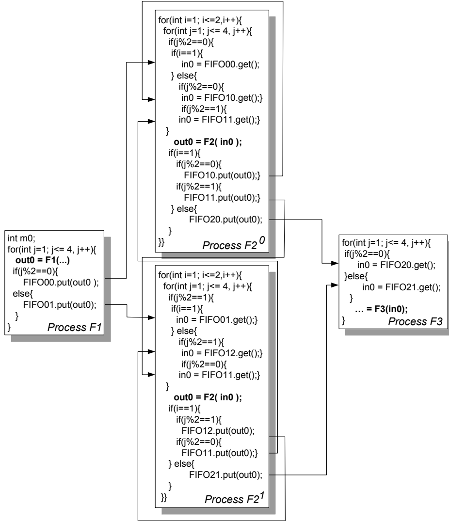
Figure 7.5: The network after process P2 was split
