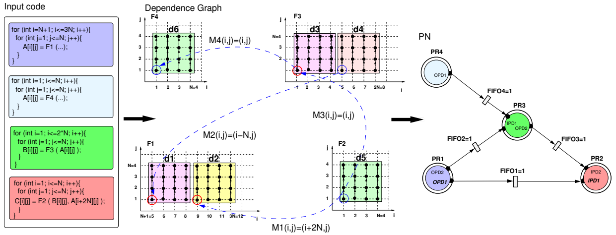
Figure 8.4: Deadlock under the conditions imposed by Theorem 7
