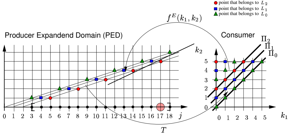
Figure 6.11: Lattice functions
