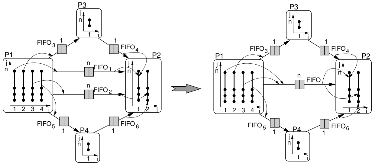
Figure 7.10: An example that shows opportunity for channel merging. We observe that FIFO_1 needs to be filled with n tokens before process P_2 can start to execute its first stage in which all tokens from FIFO_1 are consumed. Similarly FIFO_2 needs to be filled with n tokens before process P_2 can start to execute its second stage. Analyzing the flow of data through FIFO_1 and FIFO_2 (shown by arrows), we conclude that they can be merged. As a result of merging the two channels, a memory reduction of n locations is obtained.
