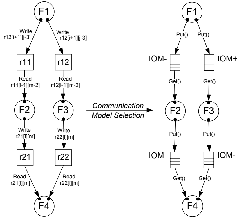
Figure 5.1: Communication Model Selection applied to the running example. See Section 5.1 for the meaning of IOM- and IOM+.
