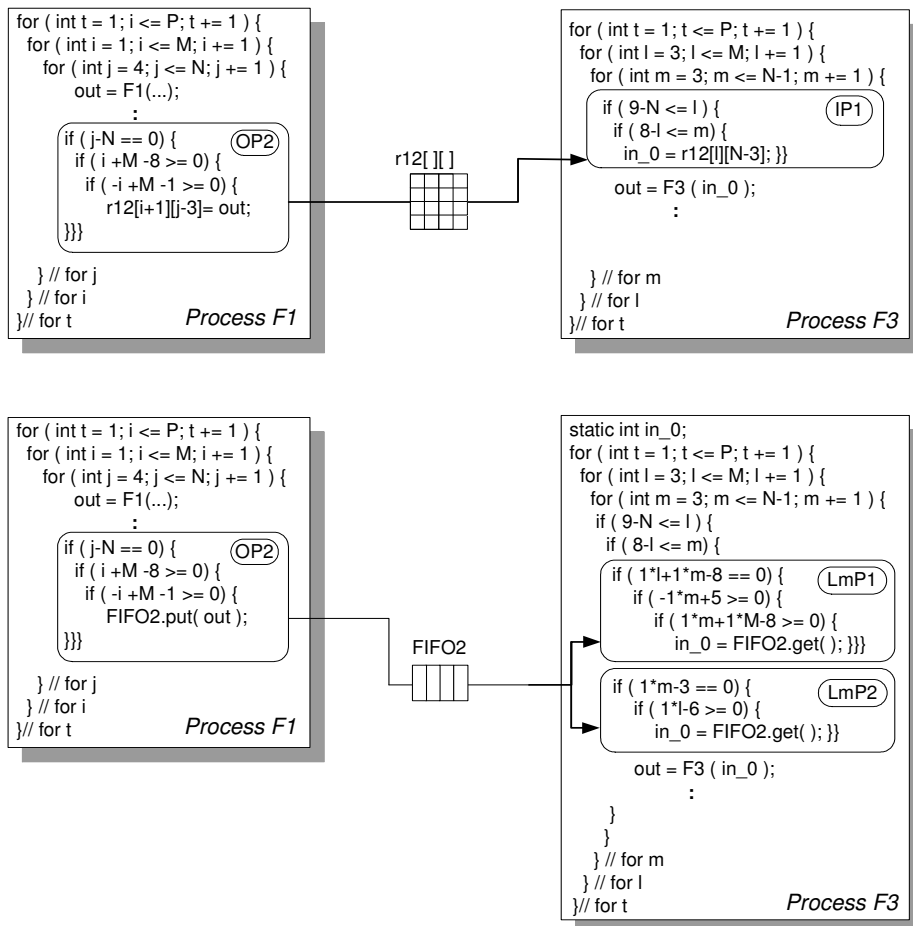
Figure 6.15: Address generation for an IOM+ P/C pair
