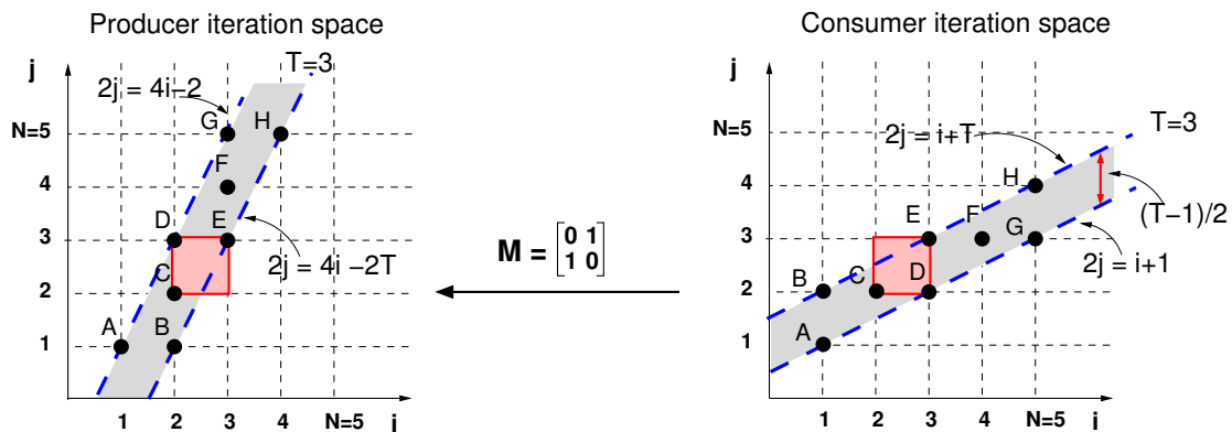
Figure 5.7: Reordering example with T = 3
