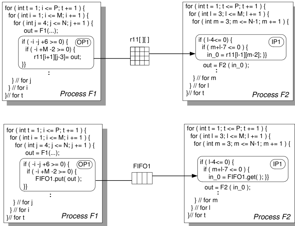
Figure 6.13: Address generation for an IOM- P/C pair
