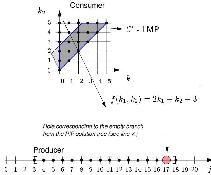
Figure 6.7: P/C iteration spaces
