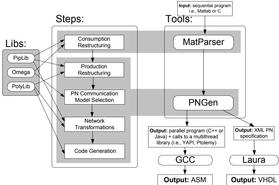
Figure 8.1: The Compaan compiler flow overview
