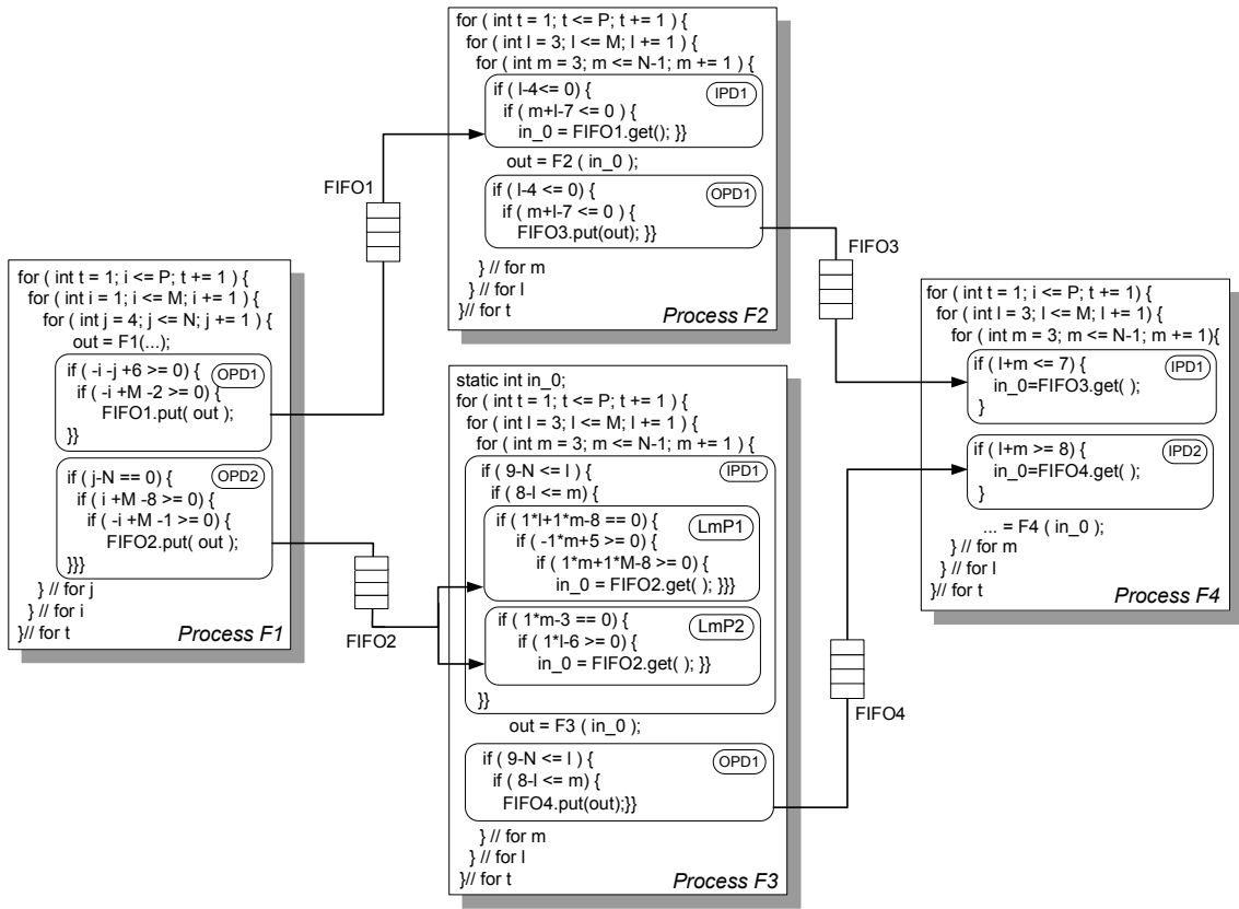
Figure 6.19: The final network implementation
