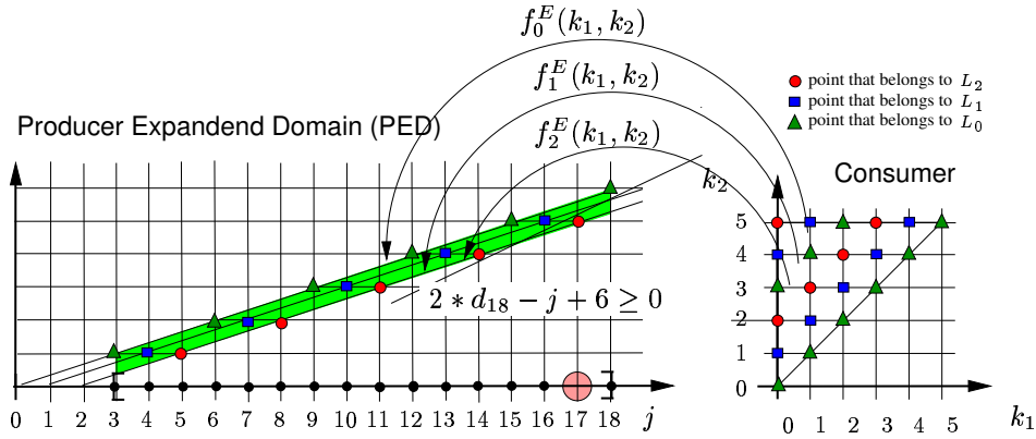
Figure 6.10: Making the dependency function explicit for each consumer lattice
