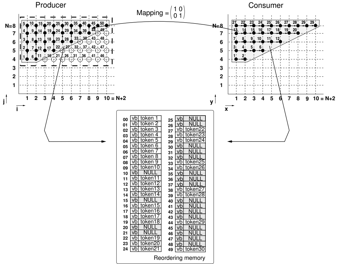
Figure 6.16: The Linear realization
