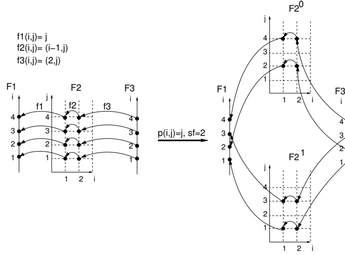
Figure 7.4: Splitting at the DDG level
