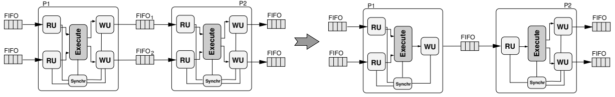
Figure 7.11: An example that shows opportunity for control reduction due to channel merging. For each FIFO we have a read control unit RU and a write control unit WU. The structure of these control units depends greatly on the implementation. For example, in a hardware implementation [113] they may contain counters used to address the FIFO locations, and automata used to check the status of the FIFO (empty or full). By merging the two FIFOs we reduce also the control units.
