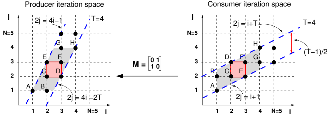
Figure 5.8: Reordering example with T = 4
