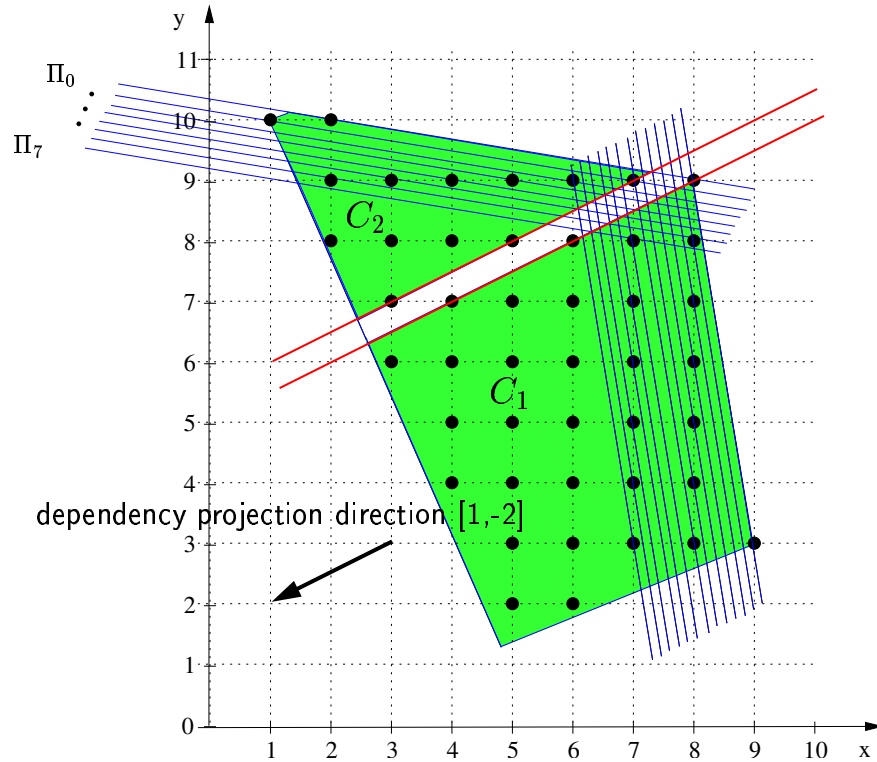
Figure 6.12: The LMP domains for a multi-domain solution tree obtained as union of planes intersected with the corresponding partition of the consumer domain. In this case the consumer is partitioned into two separated domains delimited by (red) lines.
