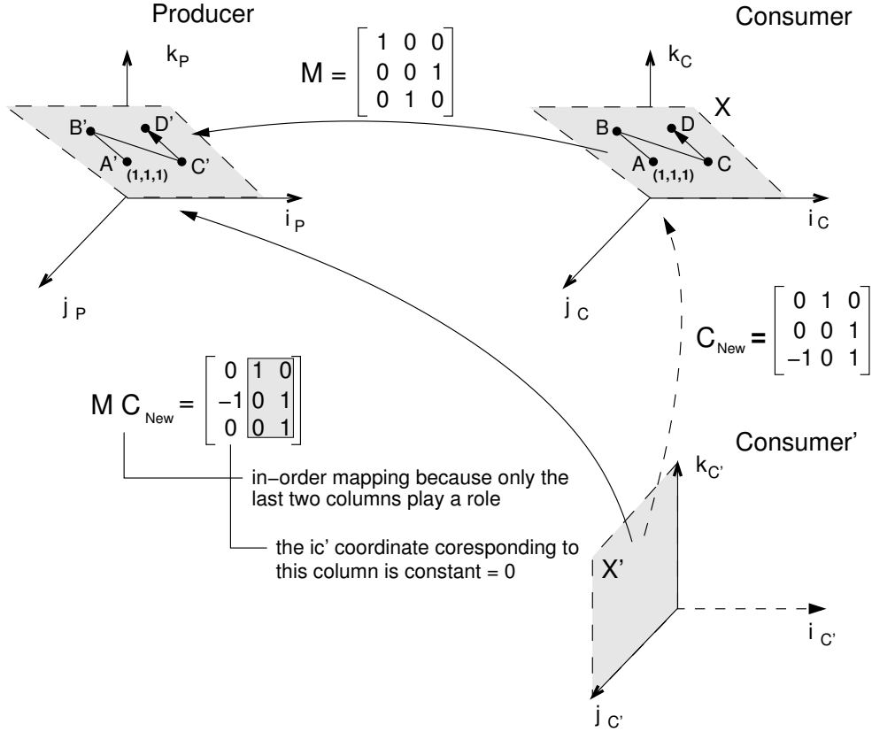
Figure 5.13: An in-order example
