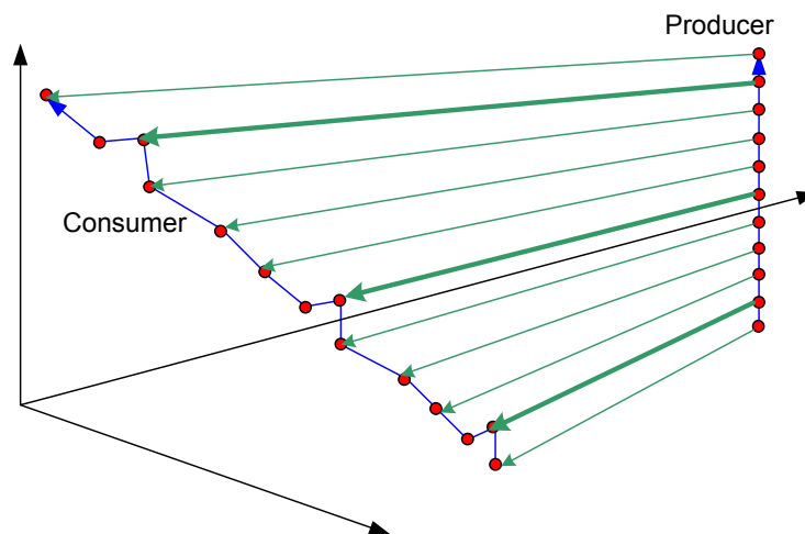
Figure 6.9: 3-D visualization of the P/C pair of Example 3; the producer domain is exposed in the back part of the picture, while the consumer is in the front. The thick horizontal lines show the multiplicity structure.
