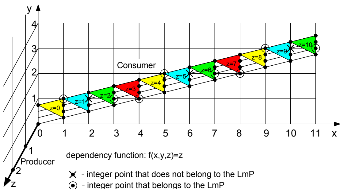
Figure 6.8: Consumer and Producer domains for P/C pair of Example 3. ILP is needed for LmP calculation.
