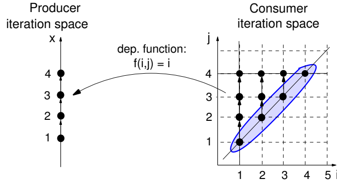
Figure 6.6: The Lexicographically Minimal Preimage for a IOM+ P/C pair
