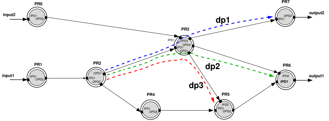
Figure 8.2: Example of a data-path in a KPN
