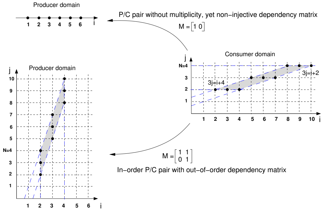
Figure 5.15: The classification requires the ILP formulation of MT and RT tests
