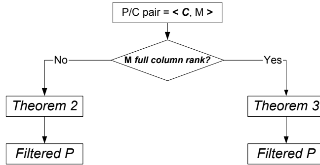
Figure 4.4: A hybrid approach that combines the ILP and the SNF approaches
