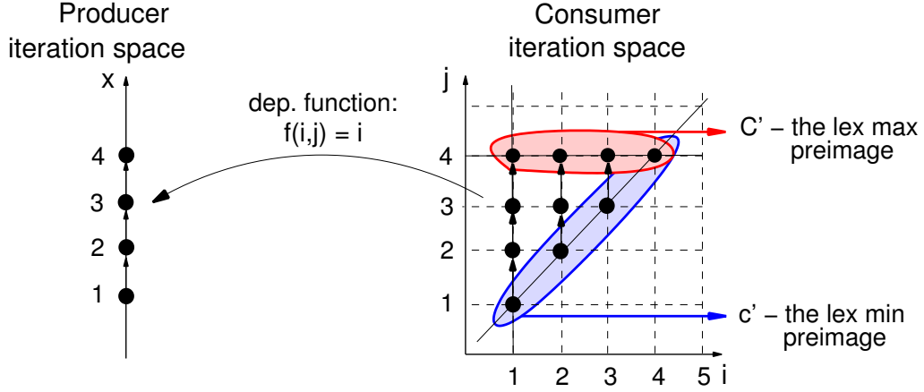
Figure 6.5: Lifetime analysis over a P/C pair with multiplicity
