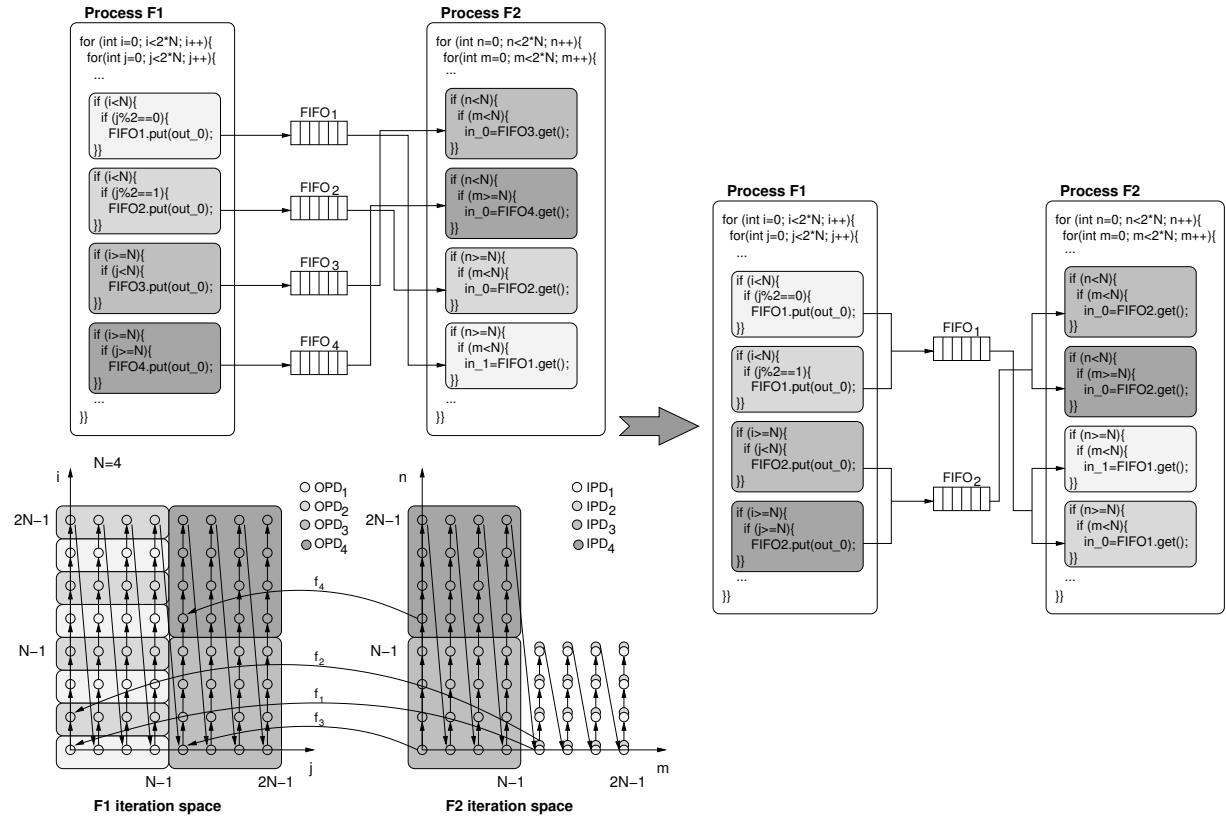
Figure 7.13: A comprehensive example showing various situations related to the in-order channel merging problem.
