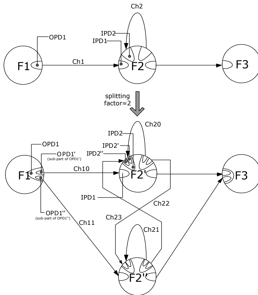
Figure 7.2: The topological aspects of splitting 2 times the process F2
