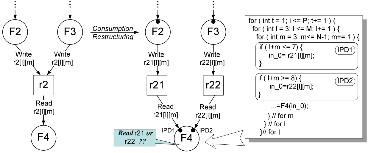
Figure 3.1: Consumption restructuring - need for dependences analysis
