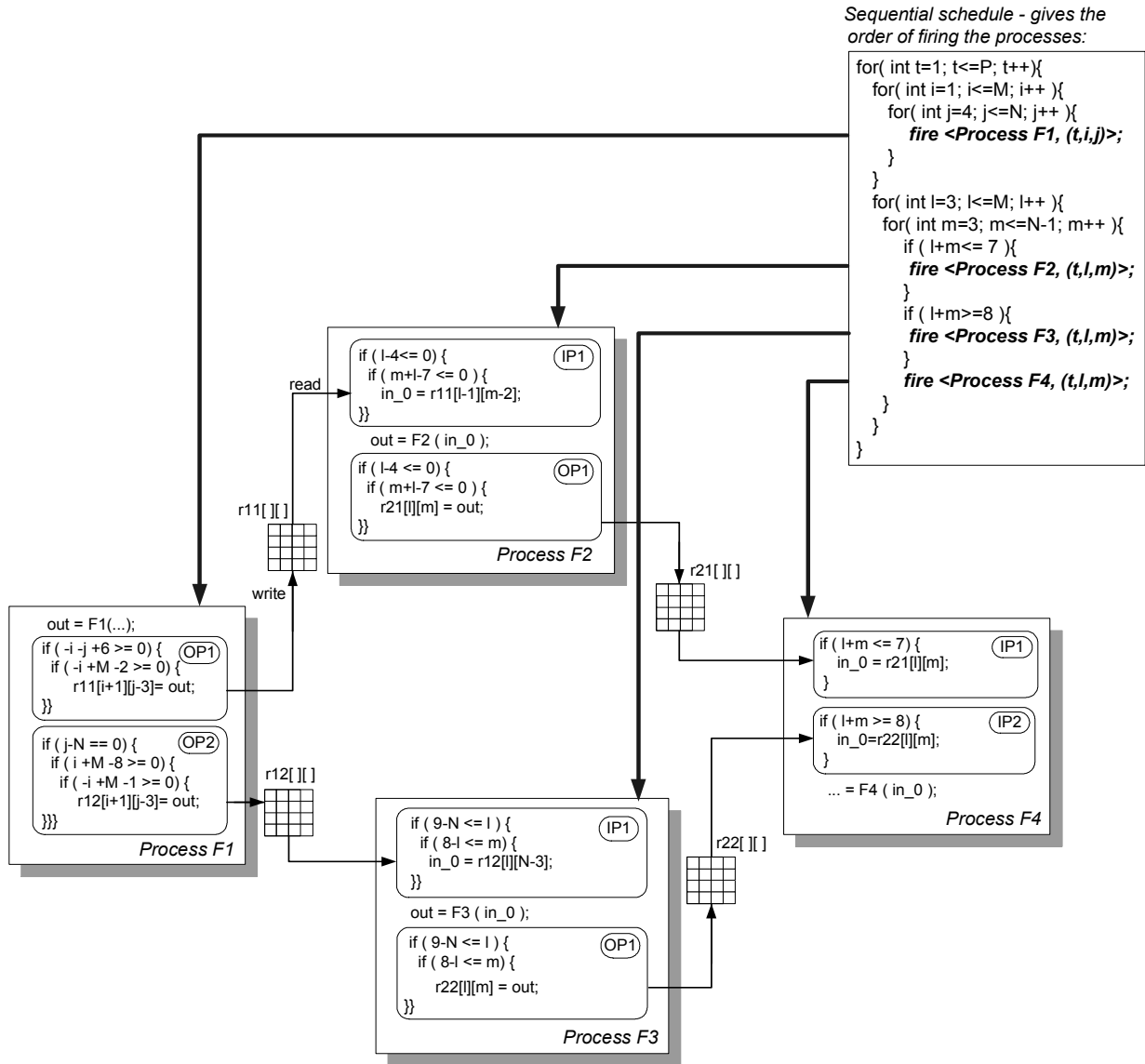
Figure 6.2: Intermediary Process Network together with a sequential schedule
