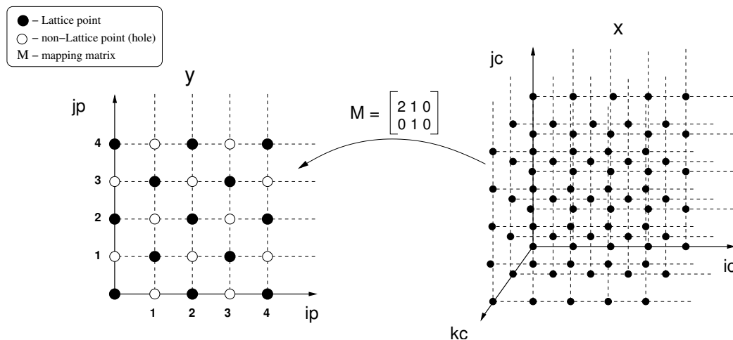
Figure 4.5: Lattice - regular holes introduced by the mapping
