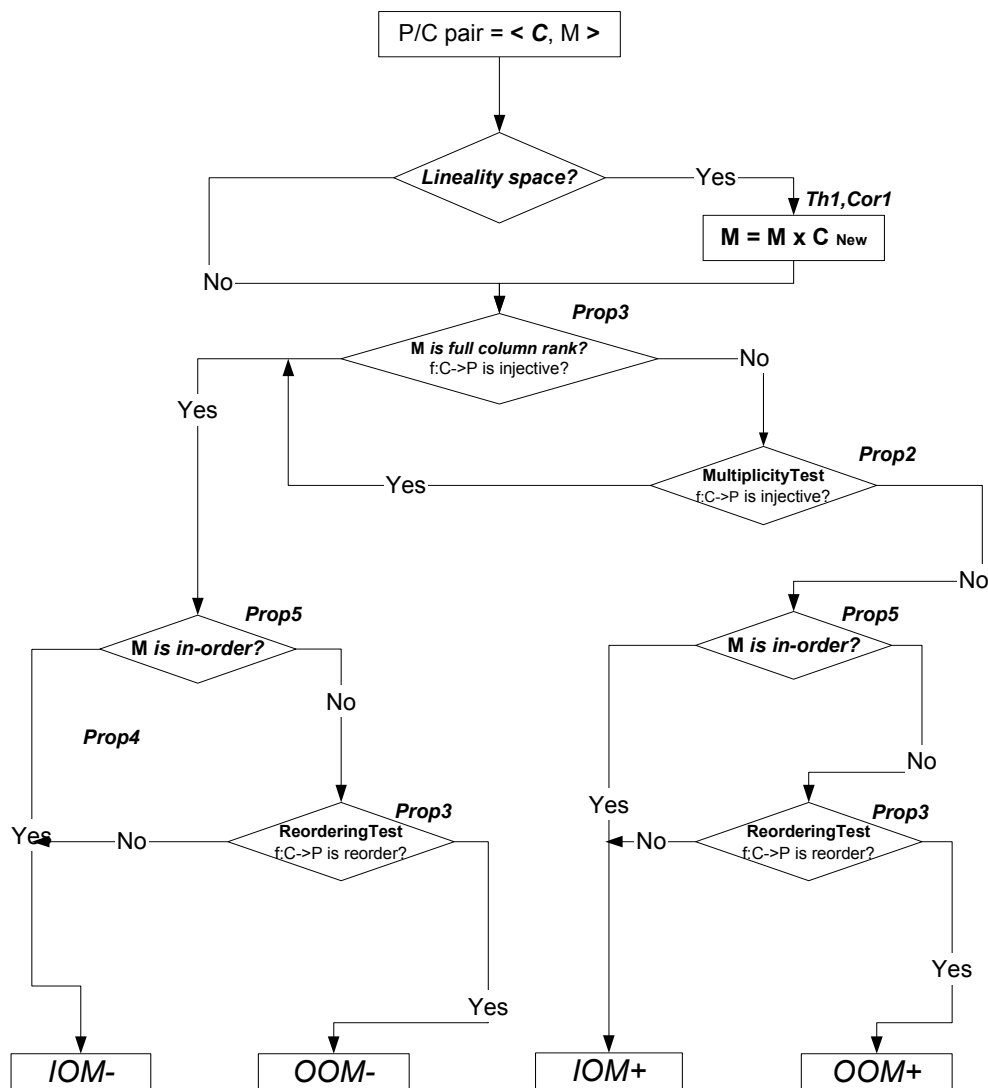
Figure 5.16: The Hybrid Reordering/Multiplicity Decision Tree
