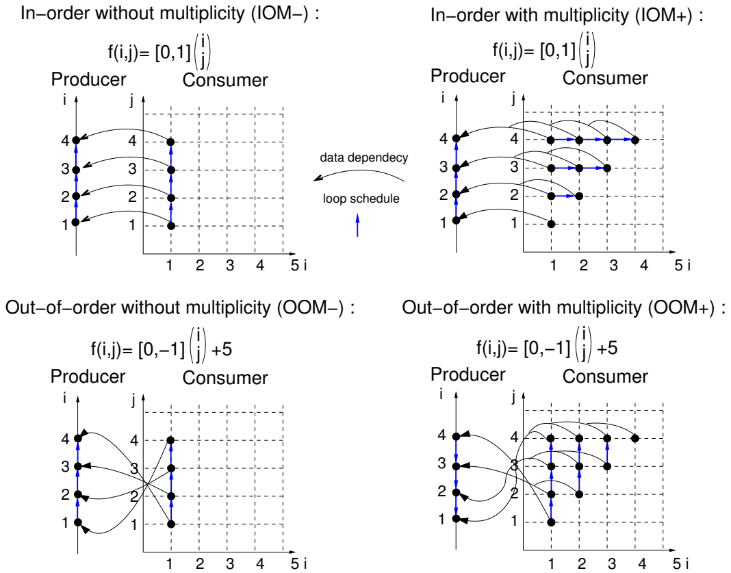
Figure 5.2: Four possible types of P/C data-flow graphs
