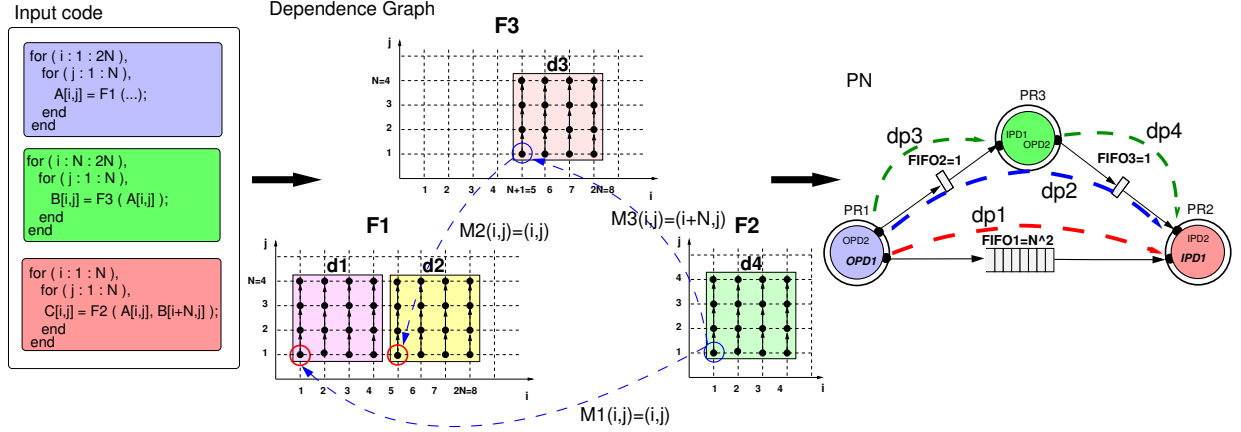
Figure 8.3: PN free of deadlock
