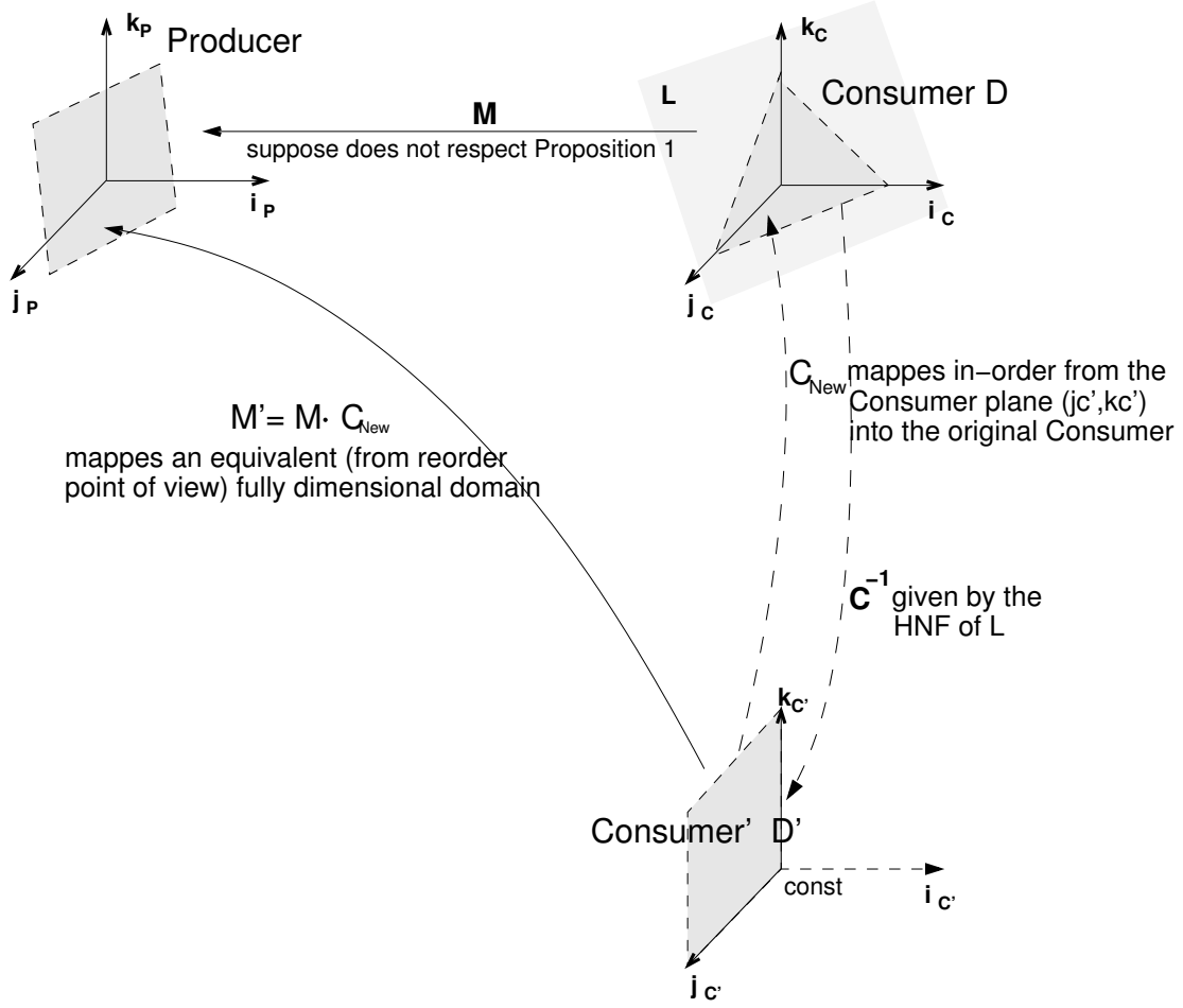
Figure 5.12: Out-of-order detection schema, when the Consumer domain has a lineality space
