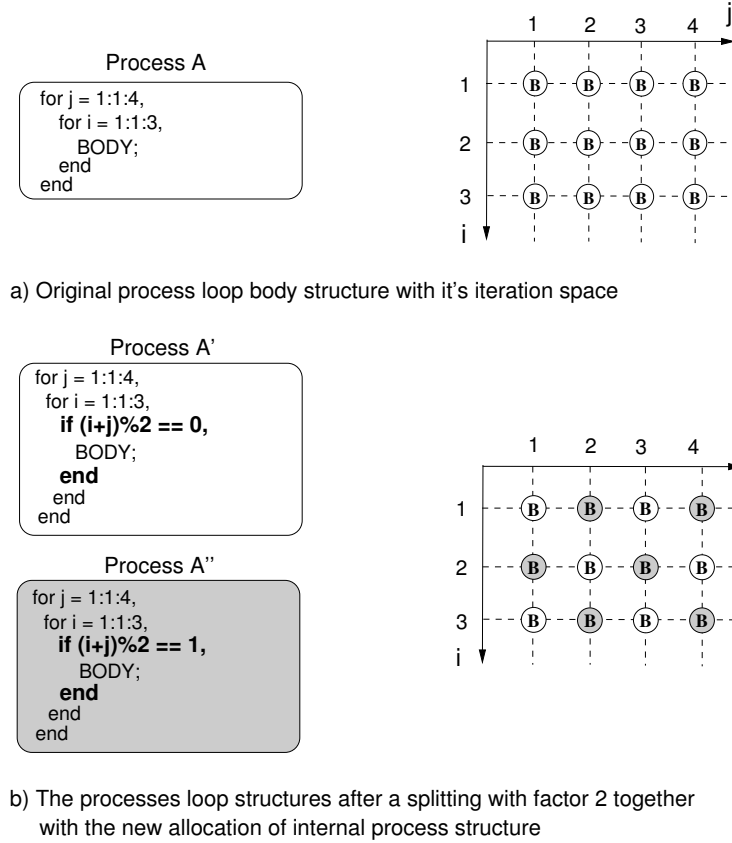
Figure 7.1: Process splitting using modulo conditional expressions
