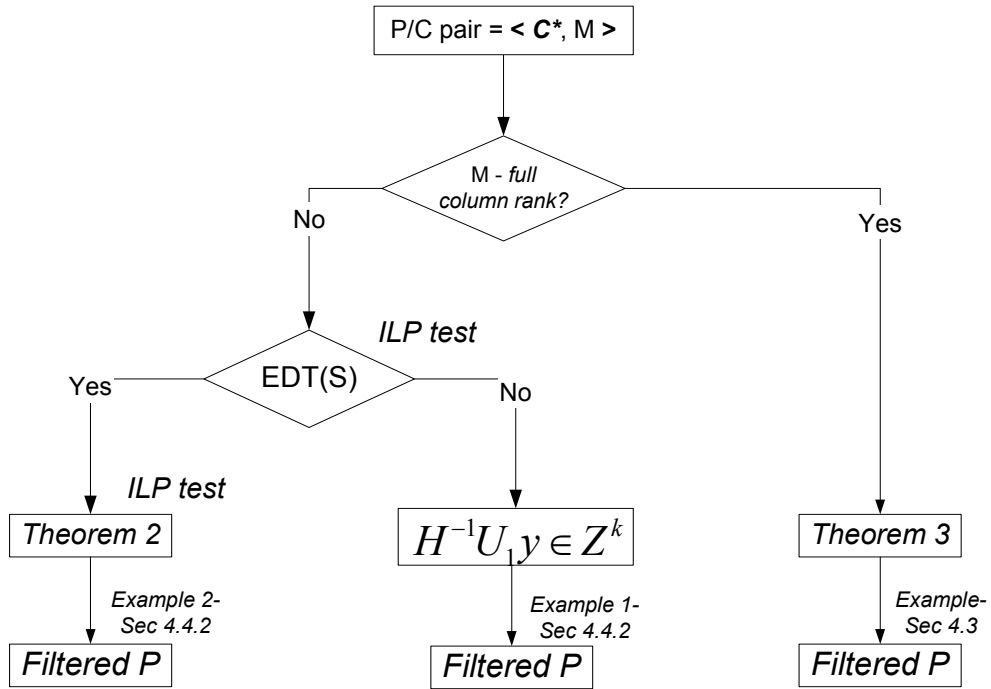
Figure 4.6: Restructuring the hybrid filtering approach
