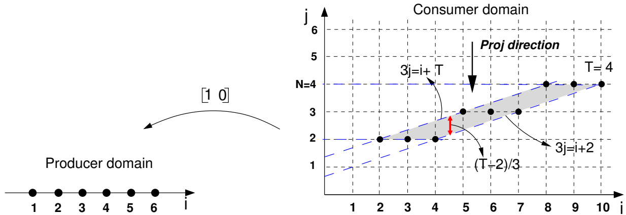
Figure 5.5: Injectivity depending on the parameters
