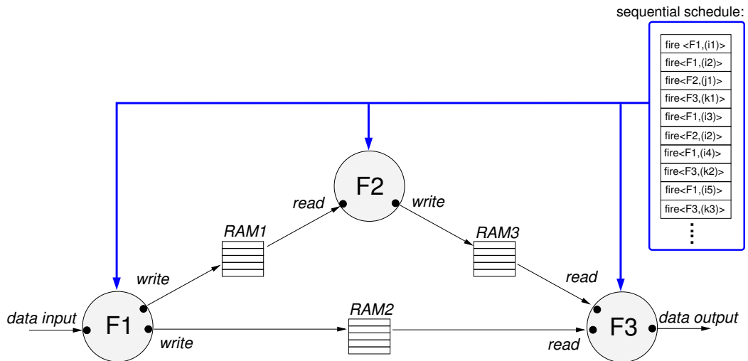
Figure 6.1: An example of an Intermediary Process Network together with the sequential schedule of firing the component processes
