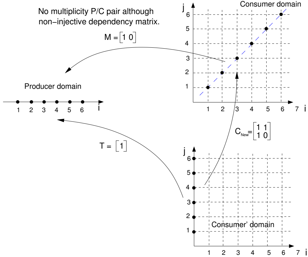
Figure 5.14: Multiplicity example with no full column rank mapping matrix
