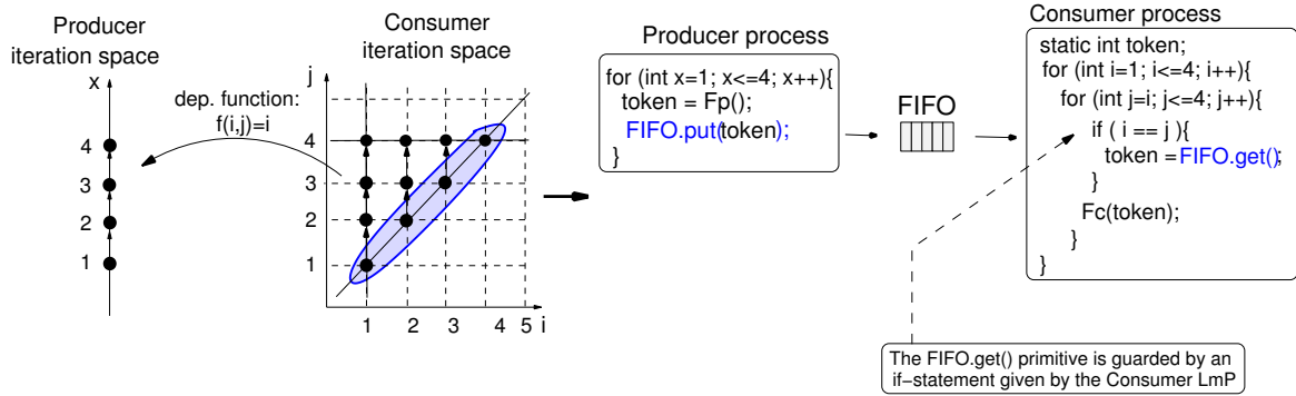
Figure 6.14: Communication for an IOM+ P/C pair
