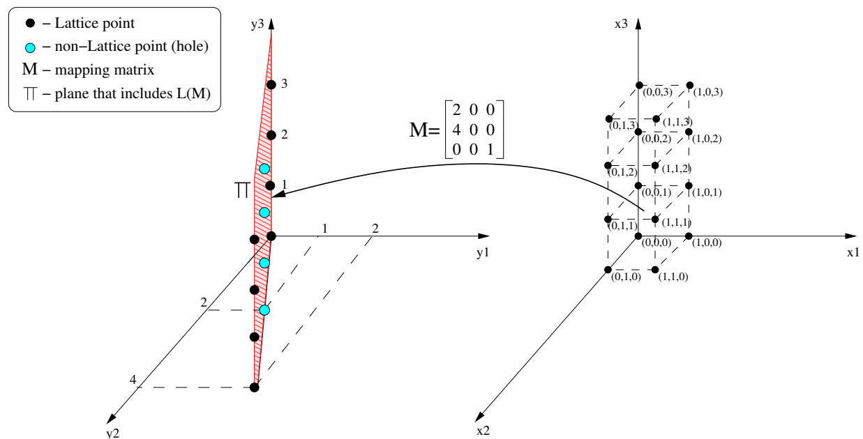
Figure 4.8: Inducing only regular holes through a non-full column rank matrix
