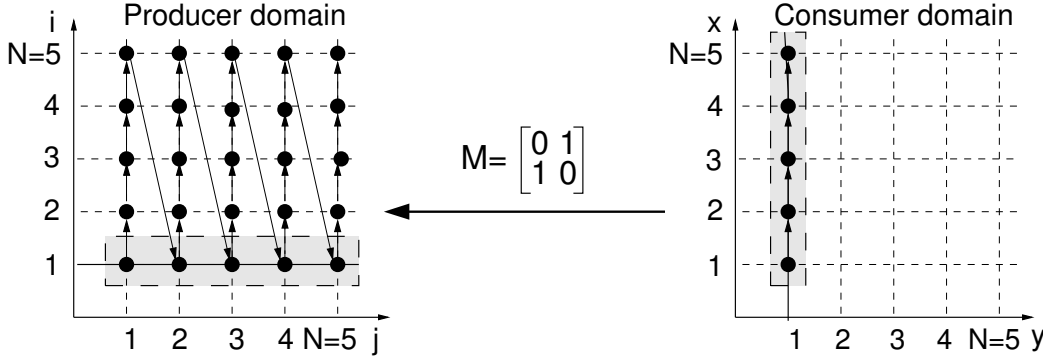
Figure 5.11: An in-order P/C pair characterized by an out-of-order mapping matrix
