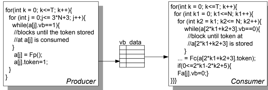
Figure 6.18: The final network implementation for OOM+
