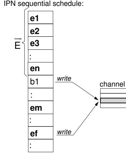
Figure 6.4: Filling the parallel PN execution into the corresponding IPN schedule
