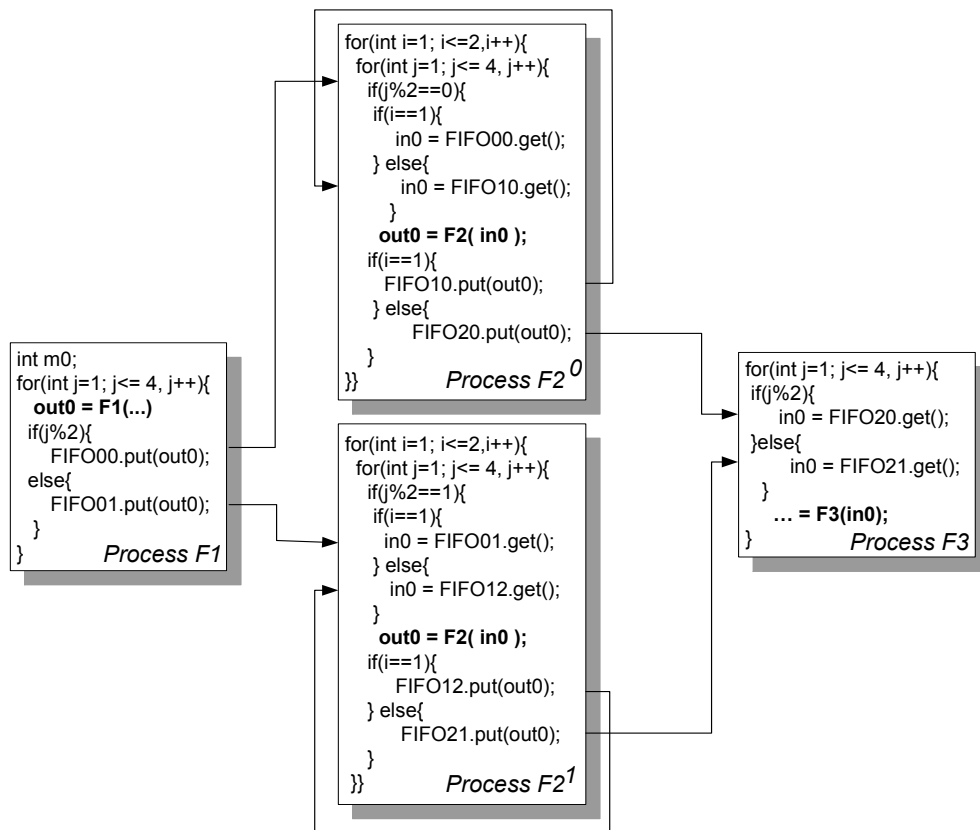
Figure 7.6: PN after removing the redundant communication
