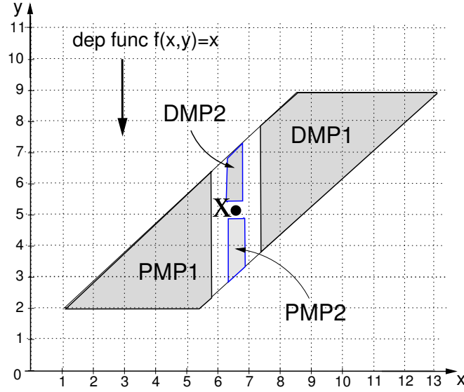
Figure 5.3: Decomposition of a domain into multiple multiplicity problems
