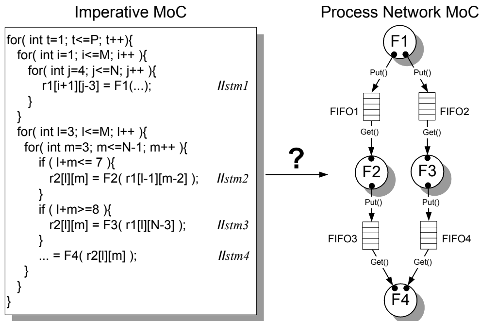
Figure 1.1: How to compile an affine nested loop application into a Process Network?
