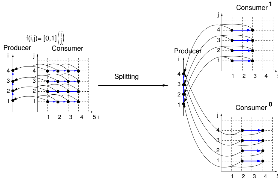
Figure 7.8: Splitting when multiplicity takes place
