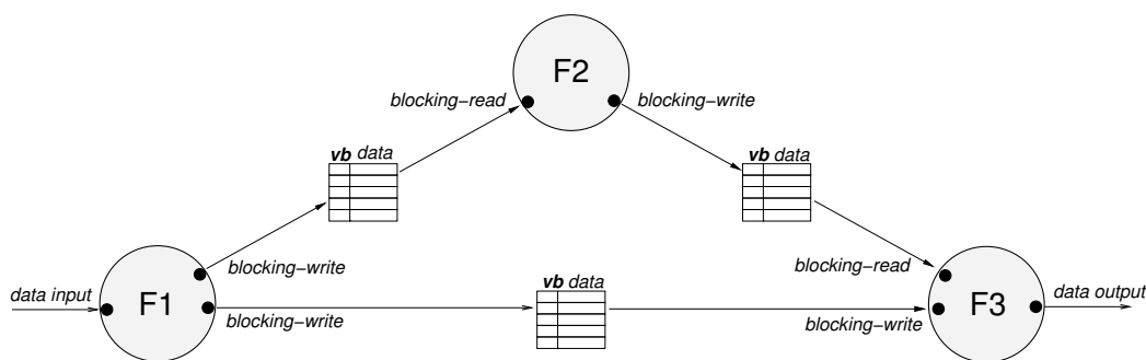
Figure 6.3: Process Network with an inter process synchronization with blocking-read and blocking-write
