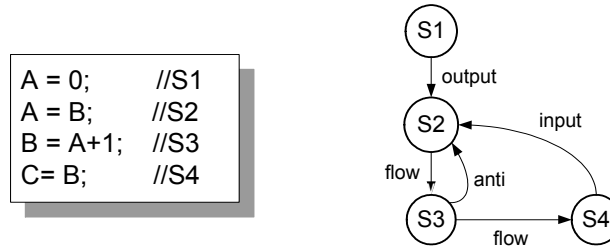
Figure 1.2: Example of a DDG
