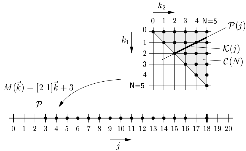
Figure 4.12: Inducing an irregular hole (i.e., j = 17 ) through a non-full column rank matrix
