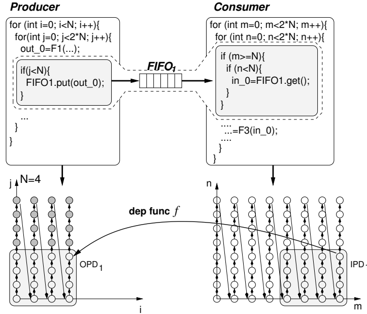
Figure 7.12: A P/C pair. For the Producer one output port domain ( OPD_1 ) and for the Consumer the input port domain ( IPD_1 ) are shown. OPD_1 is connected to IPD_1 via FIFO_1 .
