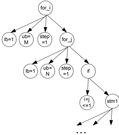
Figure 2.1: Polyhedral representations of a SANLP
