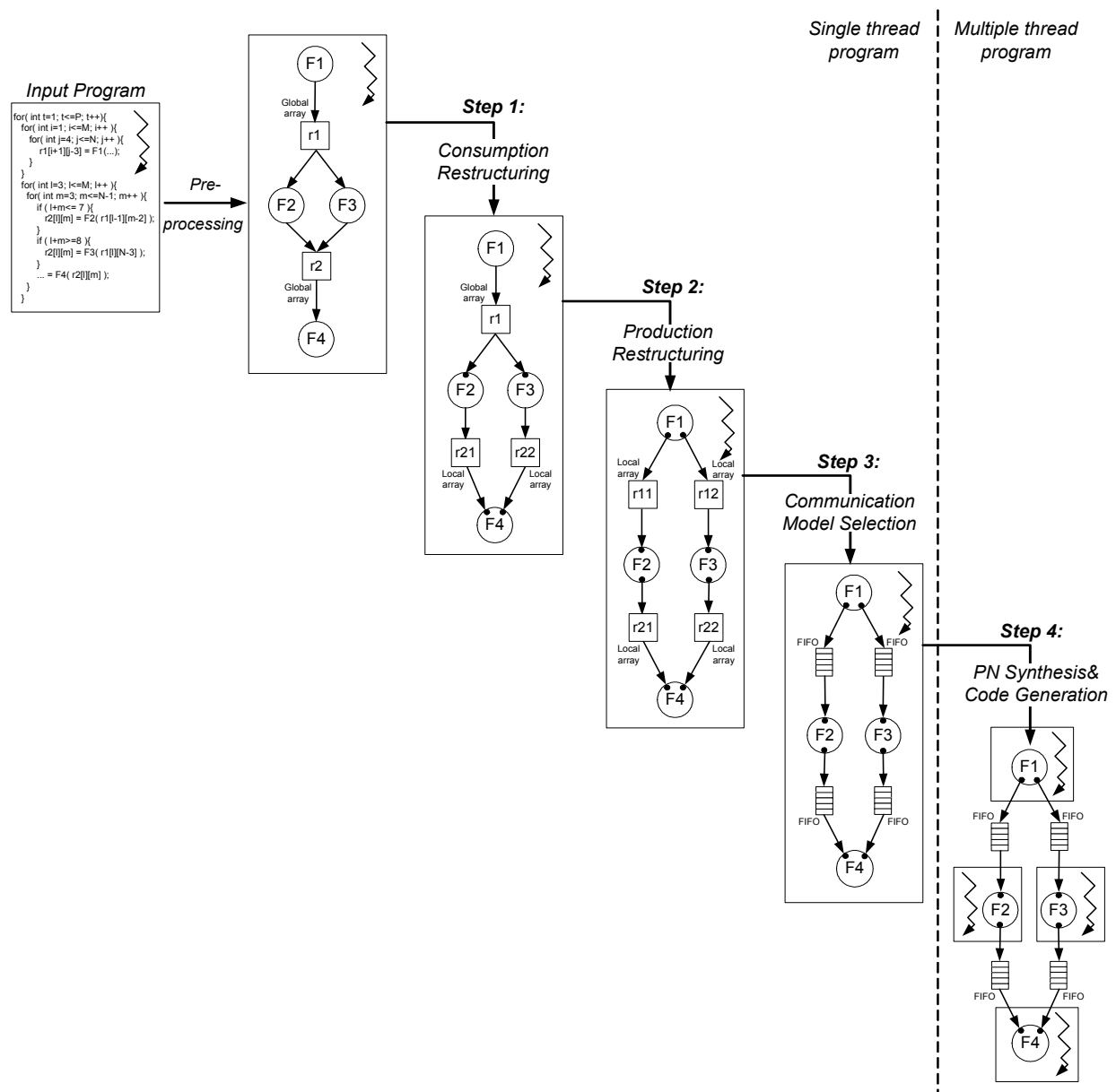
Figure 1.3: Deriving a Process Networks in four steps
