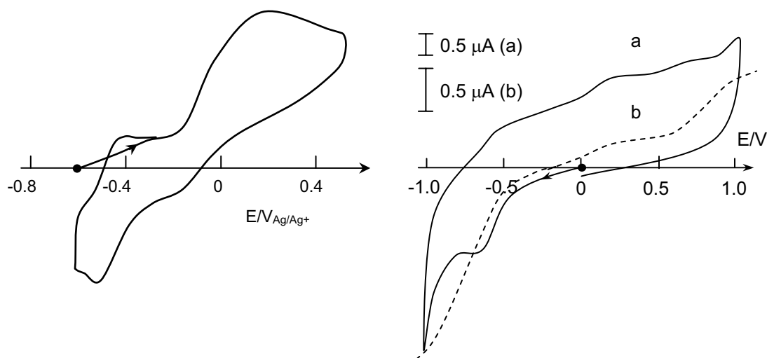
Figure 7.5. Left: CV curve recorded in a 1 mM solution of 2 in CH_3CN + 0.1 M TBAP on a Pt disc ( \varnothing = 5 mm), v = 0.1 V \cdot s ^{-1} . Right: voltammetric curve in CH_3CN + 0.1 M TBAP of the peroxo-dicopper complex 3 ( in situ , 2.5 \times 10^{-4} M, CH_3CN , -40 °C). (a) CV curve 0.1 V \cdot s ^{-1} (b) (dotted line) RDE 6000 rpm. E vs. Ag/10 mM AgNO_3 + 0.1 M TBAP in CH_3CN .
