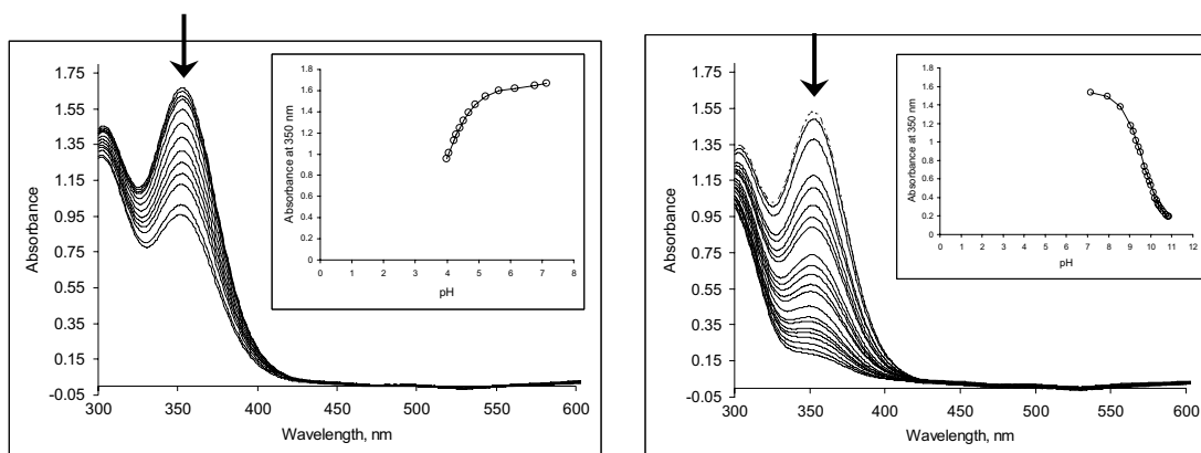
Figure 7.3. Changes in the UV-Vis spectrum of 1 upon titration with HClO 4 (left, pH range 7.1 – 4.0) and NaOH (right, pH range 7.1 – 10.9). The insert shows the decrease in absorption of the LMCT band at 350 nm vs. pH of the solution.
