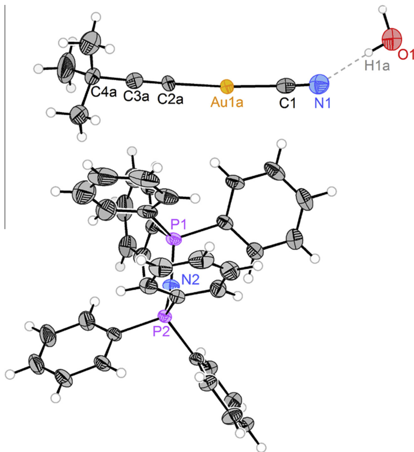
Fig. 2. Projection of cation, anion and lattice solvent molecules in compound 2 with thermal ellipsoid plot at the 50% levels of probability. Only the main component (65% occupancy) of the disordered part is depicted. Selected bond lengths [Å] and angles [°] are: Au1a–C1 2.003(4), Au1a–C2a 2.013(8), C1–N1 1.122(5), C2a–C3a 1.199(12), C3a–C4a 1.465(11), N1···O1 2.900(8), P1–N2 1.582(2), P2–N2 1.586(2), C1–Au1a–C2a 174.6(3), P1–N2–P2 135.29(17).
