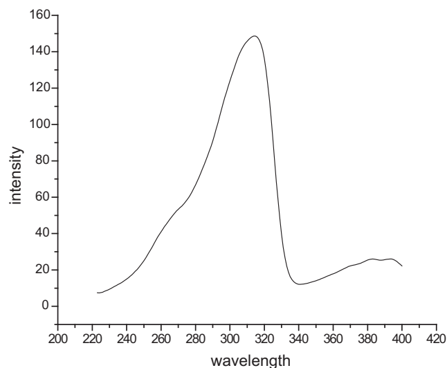
Fig. 4. Excitation spectrum of compound 1 (monitored at 431 nm).
