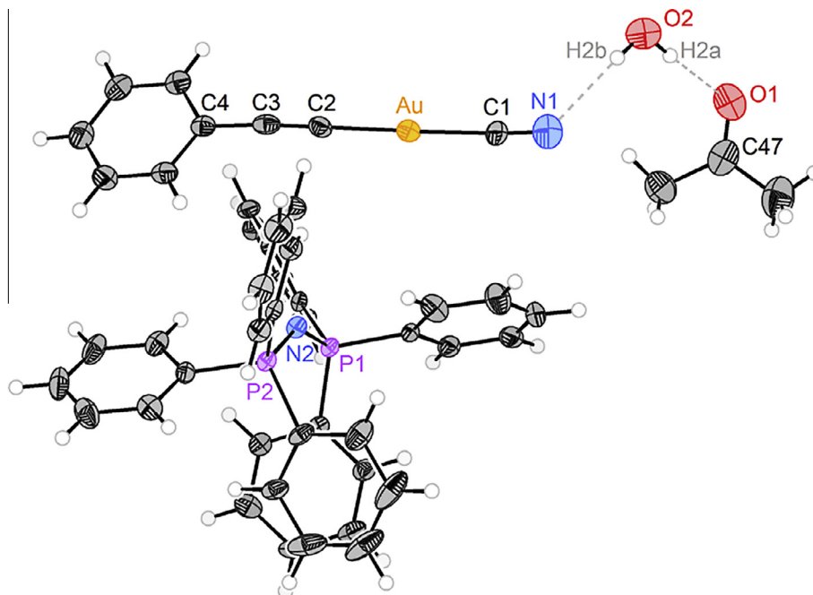
Fig. 1. Projection of cation, anion and lattice solvent molecules in compound 1 with thermal ellipsoid plot at the 50% levels of probability. Selected bond lengths [Å] and angles [°] are: Au–C1 1.971(6), Au–C2 1.990(5), C1–N1 1.158(8), C2–C3 1.204(7), C3–C4 1.429(7), N1...O2 3.009(8), O1...O2 2.921(8), P1–N2 1.580(3), P2–N2 1.584(3), C1–Au–C2 179.0(2), P1–N2–P2 136.4(2).
