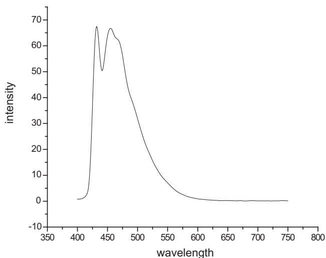
Fig. 3. Emission spectrum of compound 1 (excited at 310 nm).
