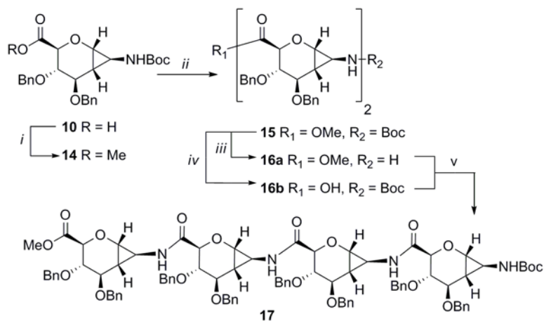
Scheme 4. Synthesis of a homotetramer of SAA 10 .
