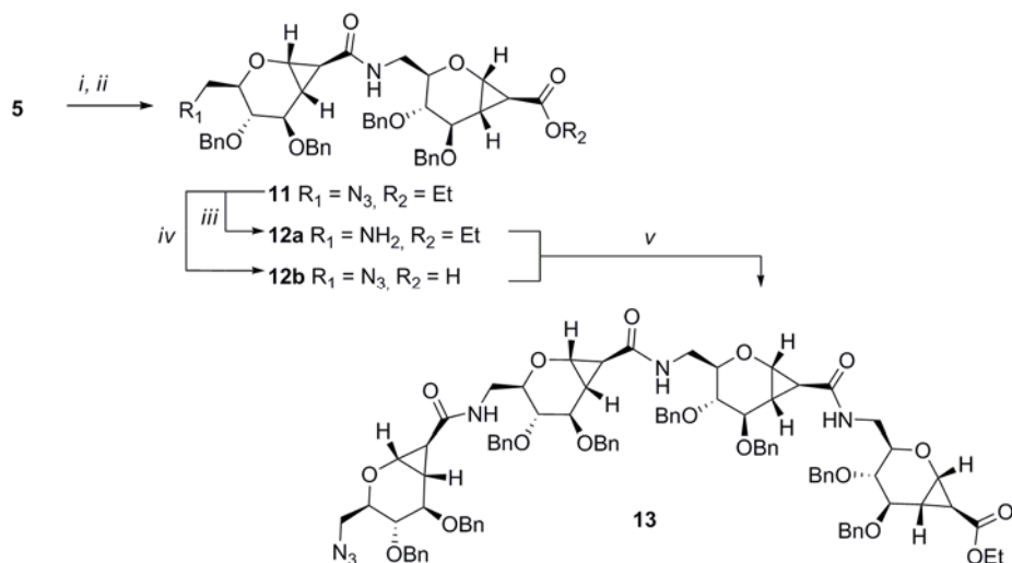
Scheme 3. Synthesis of a homotetramer of SAA 5 .
