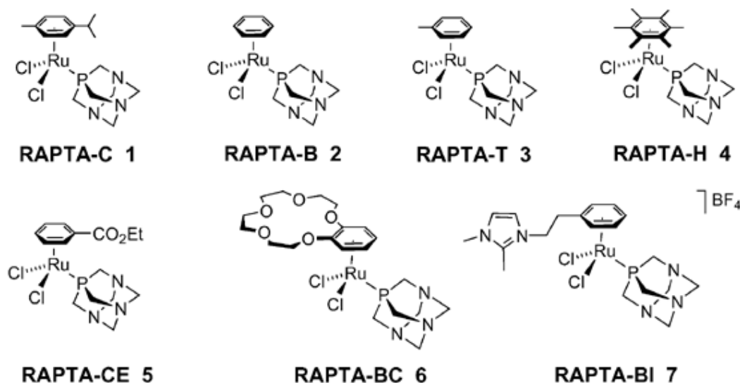
Figure 1.6.11 Schematic representation of some selected RAPTA-Ru(II)-arene analogues [196].
