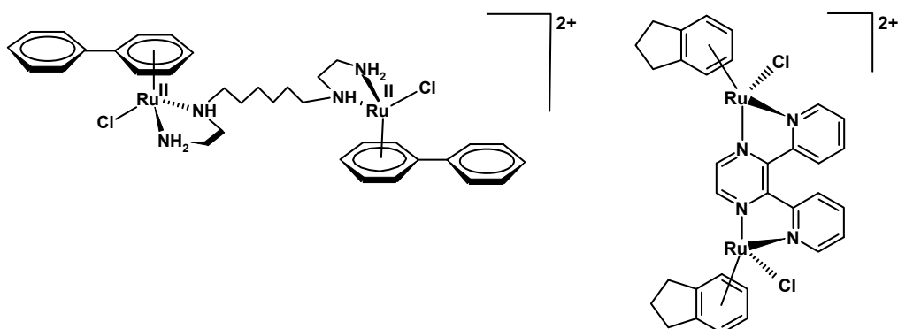
Figure 1.6.10 Schematic representation of dinuclear Ru(II)-arene analogues.
