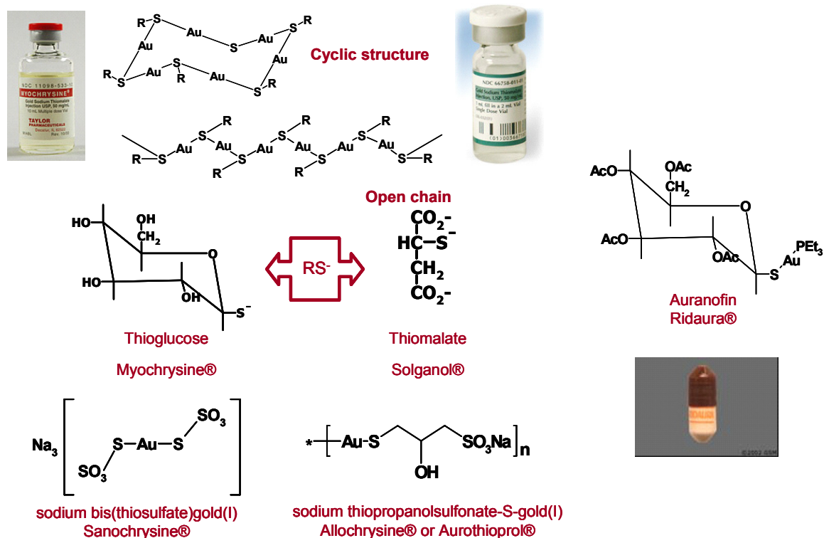
Figure 1.5.1 Schematic representation of main crysotherapy drugs commercially available [86].
